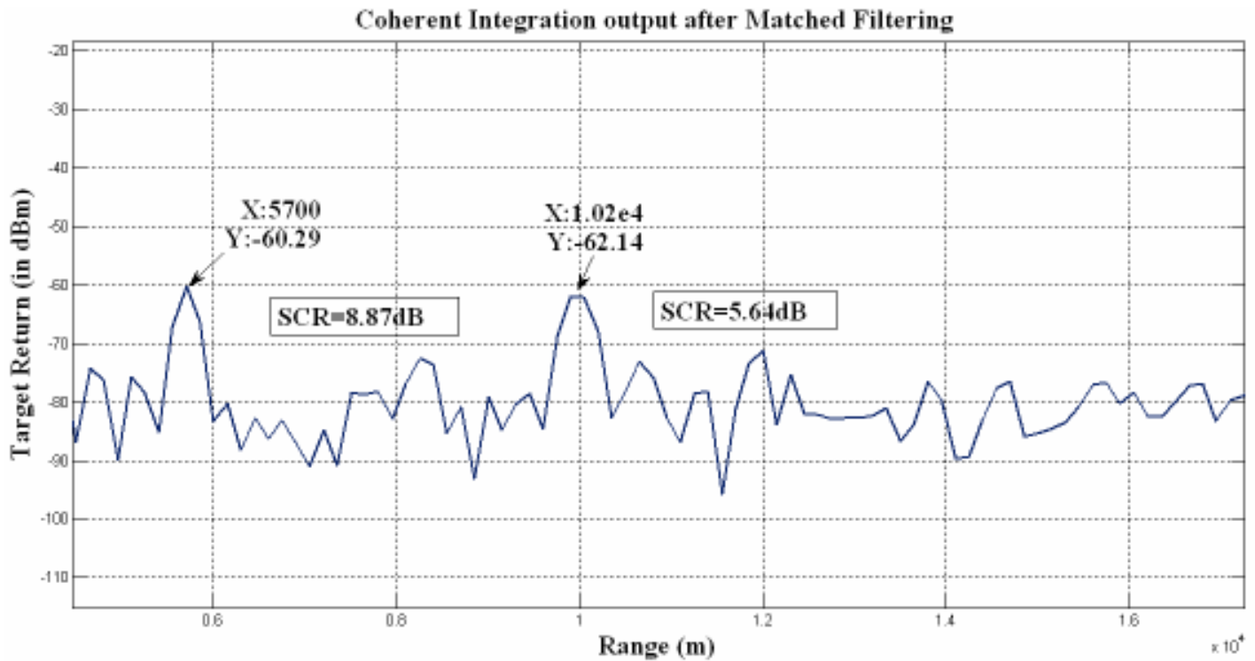
Fig.-8.6: For RCS = 0.07 \text{ m}^2
