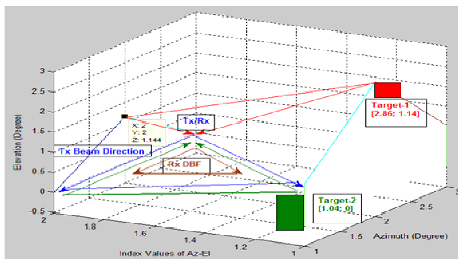
Fig.- 6: Beam Directions of TX/Rx and Target Returns.
