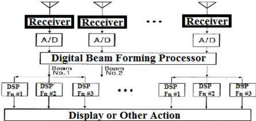
59 60 Fig1: Multi DSPs involved in Receiver Digital Beam Formation
