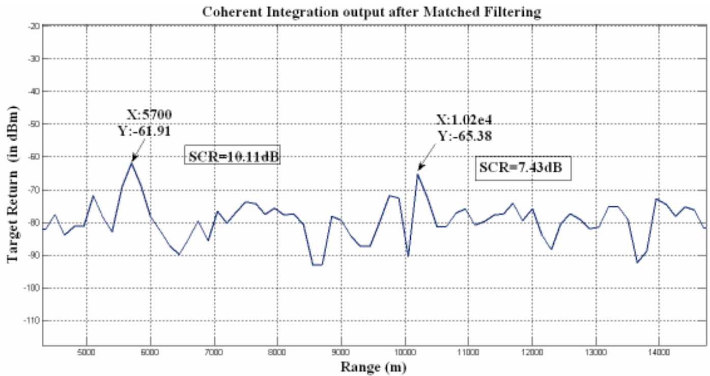
Fig.-8.5: For RCS = 0.4 \text{ m}^2
