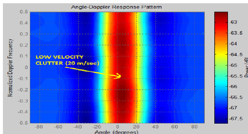
Fig.- 7 : Low velocity clutter of 20 m/sec
