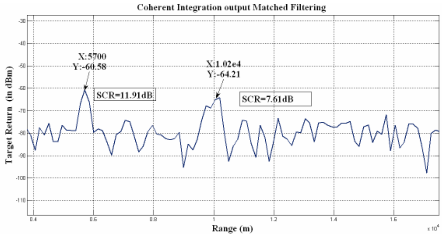
Fig.-8.4: For RCS = 0.6 \text{ m}^2
