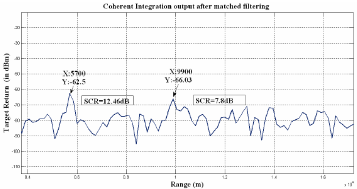
Fig.-8.3: For RCS = 0.8 \text{ m}^2
