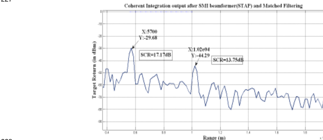
Fig.-4: Coherent Pulse Integration Output after Receiver Digital Beamformer and Matched Filtering
