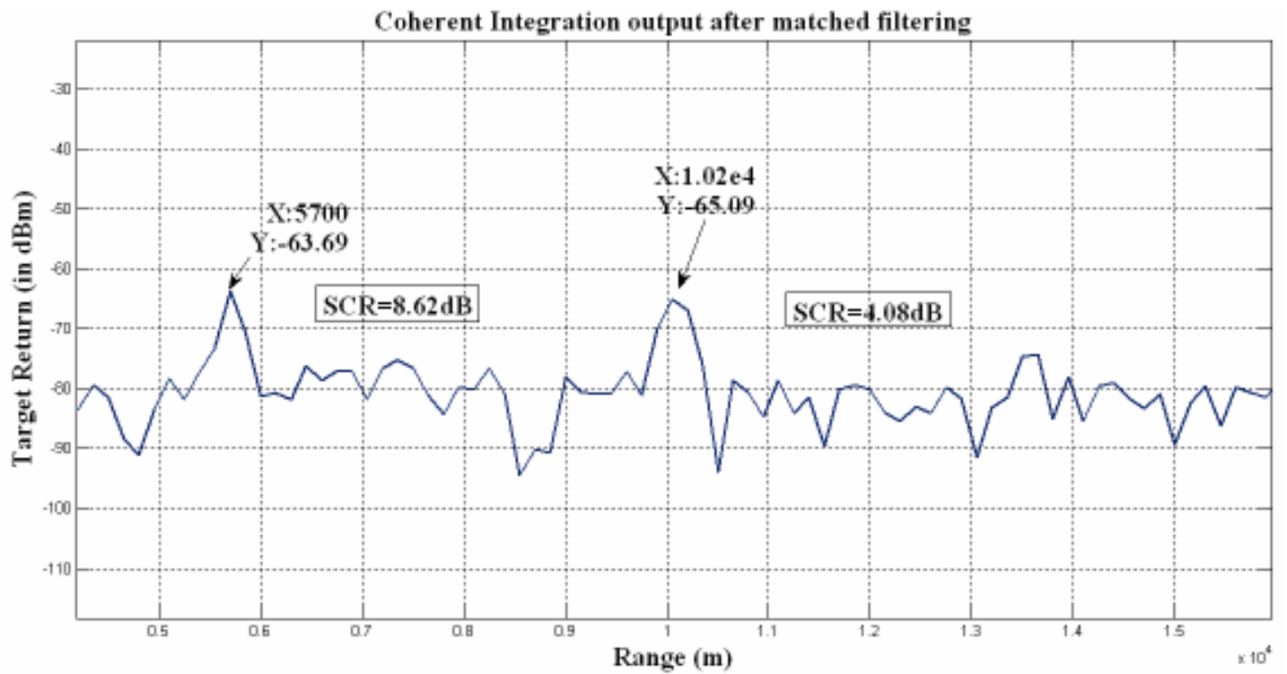
Fig.-9: For RCS = 0.04 m 2
