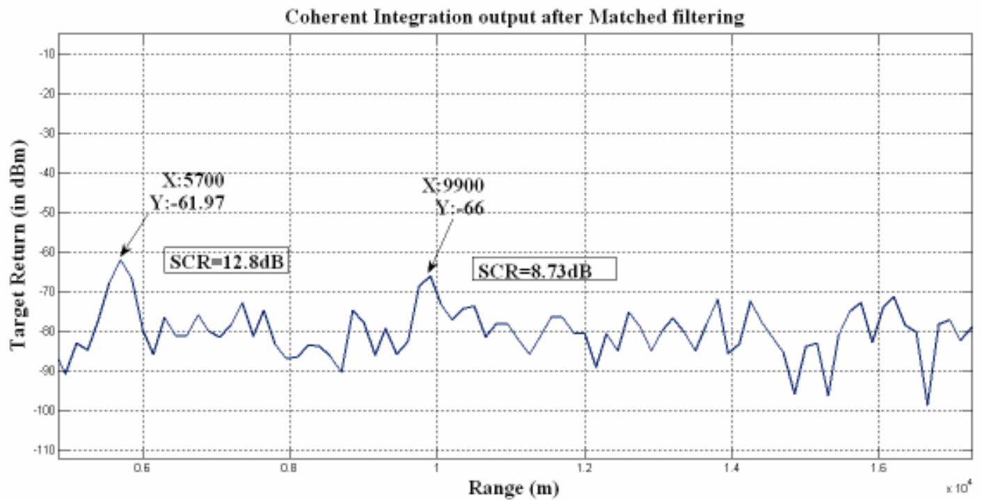
Fig.-8.2: For RCS = 1 m²
