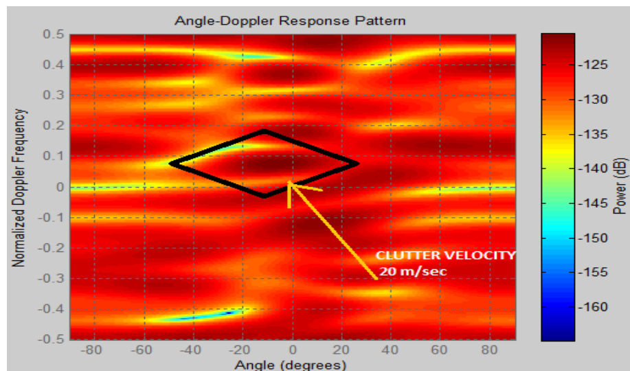
Fig.- 5: Angle-Doppler Response for low Clutter Velocity = 20 m/sec
