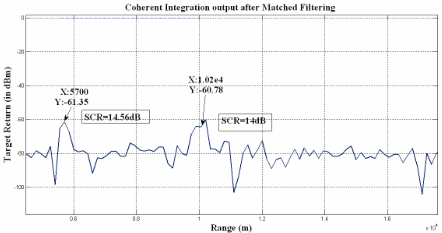
Fig.-8.1: For RCS = 1.1 m²
