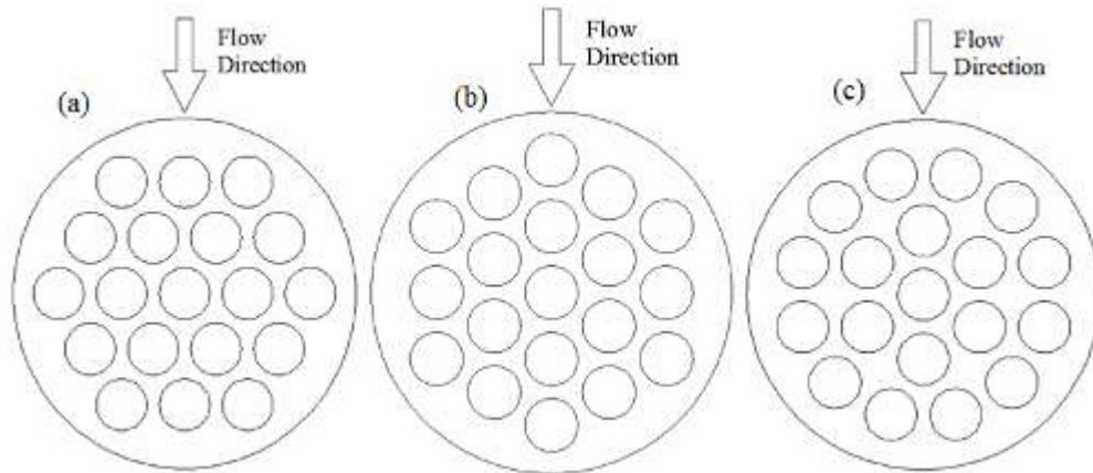
Fig. 2. Tube Bundle Arrangement for (a) triangular (STHE_T), (b) rotated triangular (STHE_RT), and (c) combined (STHE_C) patterns
