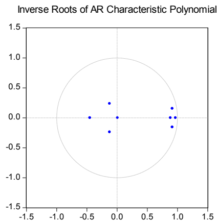
Fig.1.AR Roots in financial crisis period
