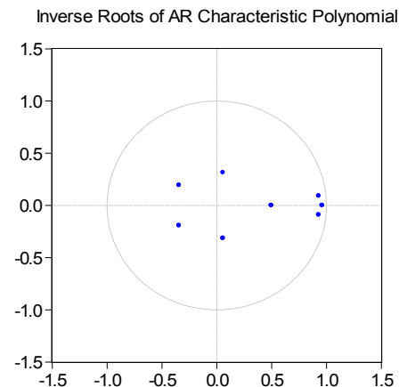
Fig.2.AR Roots in non-financial crisis period
