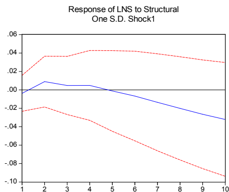
Fig.4.Response Curve of output shocks on stock price
