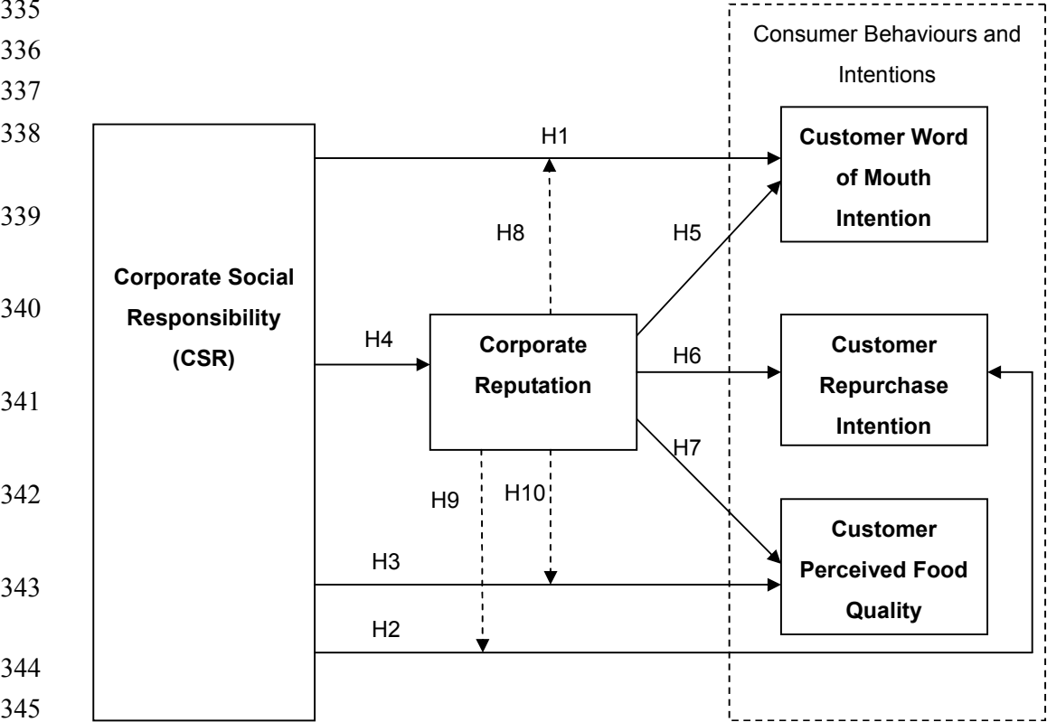
Figure 1. Research Model
