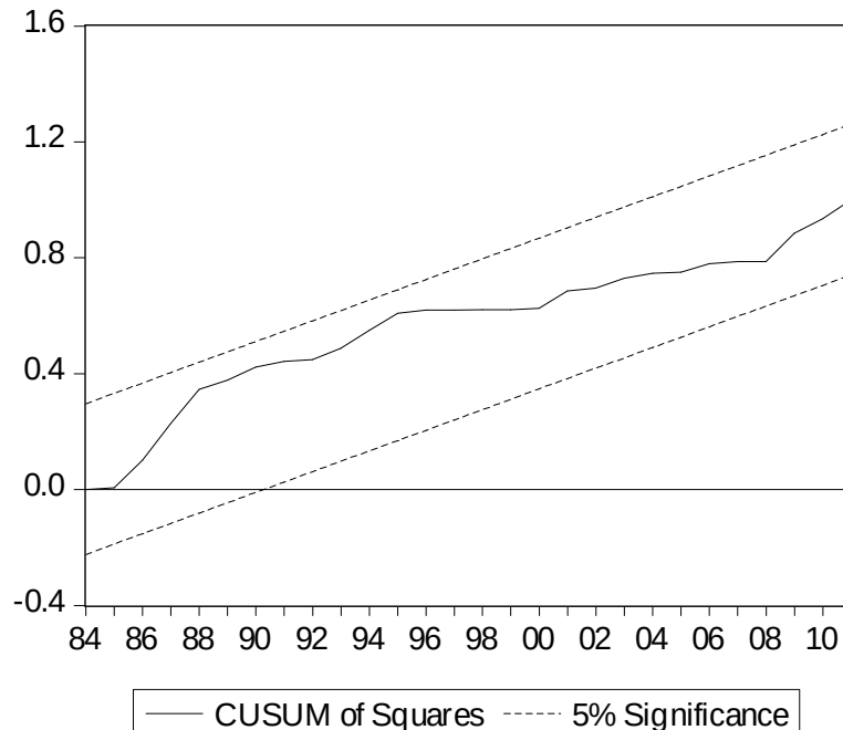
Fig. 4. Stability test for residuals
