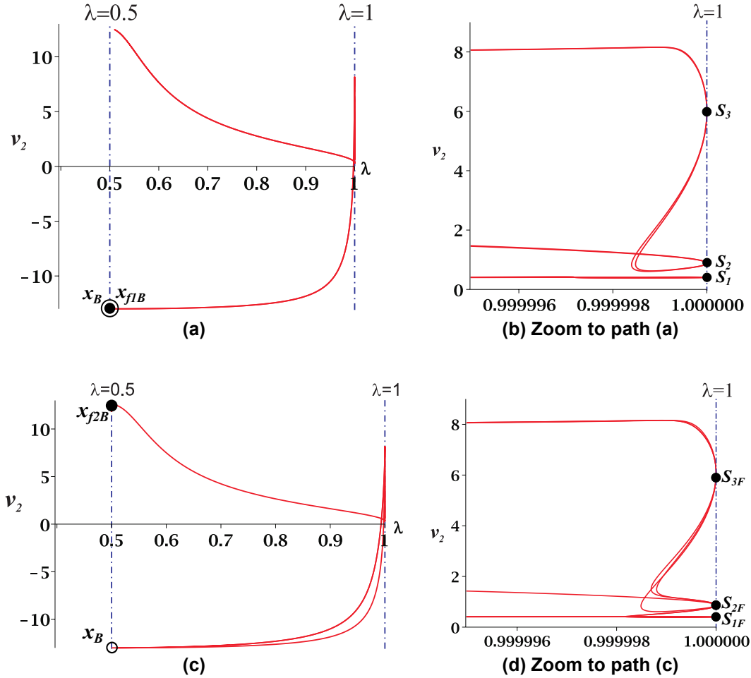
Figure 5: Homotopy paths \lambda - v_2 for initial point at x_B : (a), (b) the fault-free circuit and (c), (d) fault circuit.
