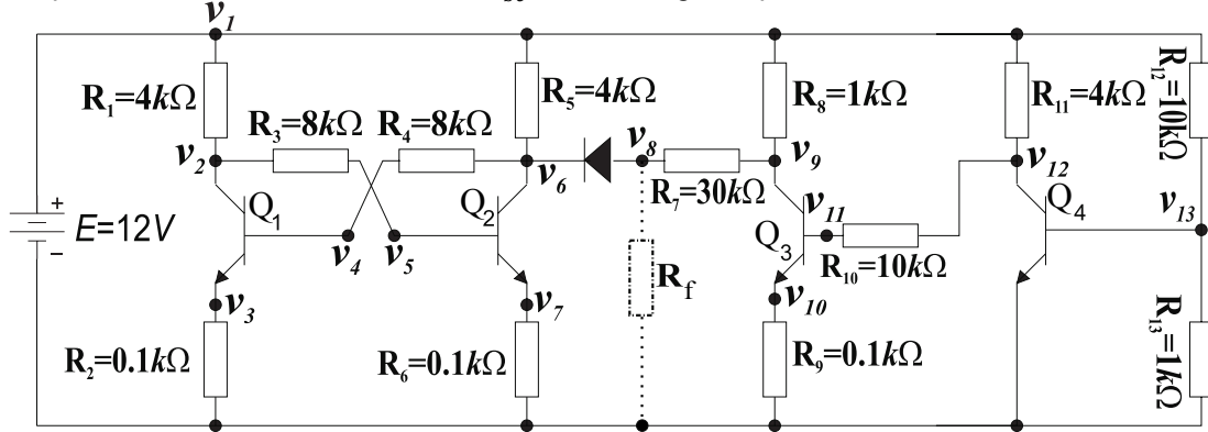
Figure 3: Circuit under test (contains three operating points). R_f = 11k\Omega models a possible fault between node v_8 and ground.
