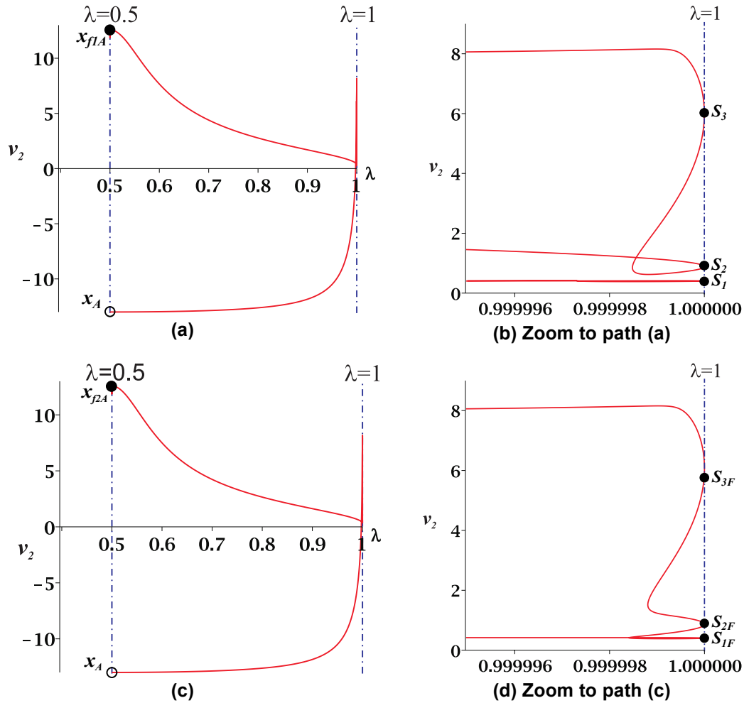
Figure 4: Homotopy paths \lambda - v_2 for initial point at x_A : (a), (b) the fault-free circuit and (c), (d) fault circuit.
