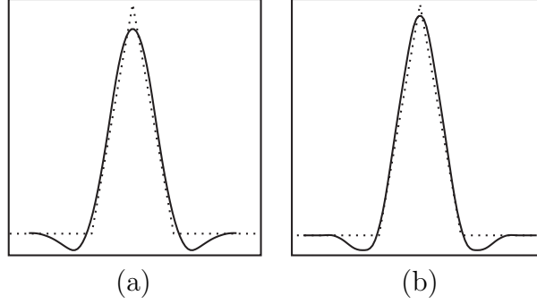
Figure 1: (a) and (b) present basic function of proposed schemes (3.3) and (3.4) respectively.
