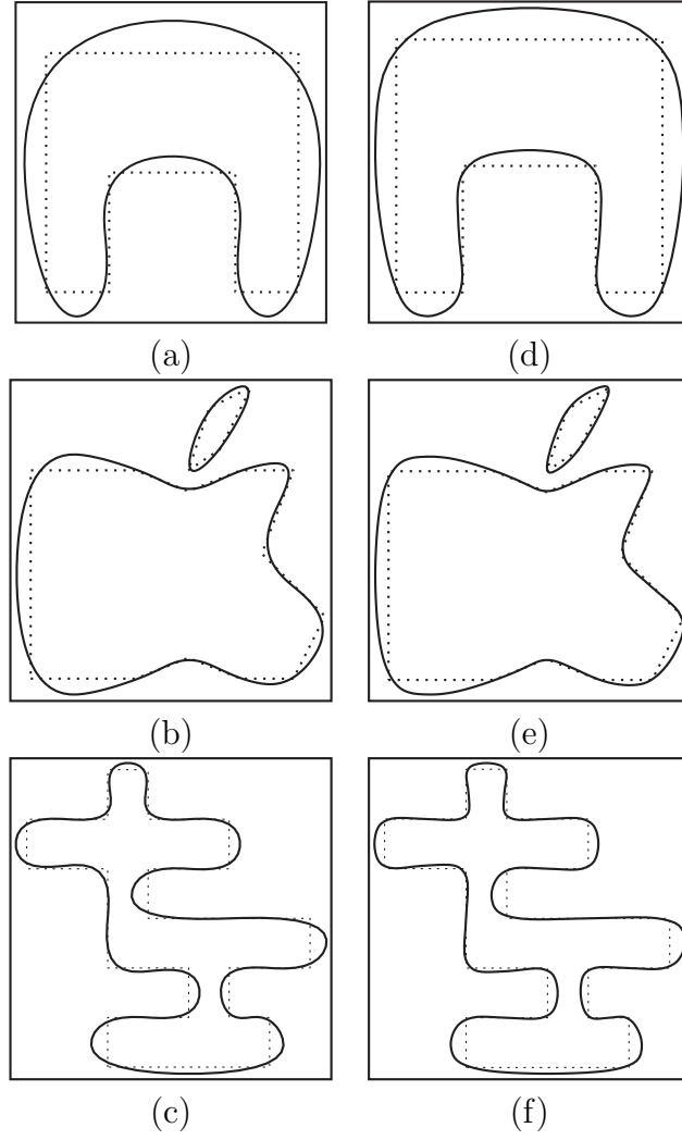
Figure 2: (a)-(c) present limit curve of the scheme (3.3) after 4th subdivision level and (d)-(f) present limit curve of the scheme (3.4) after 2nd subdivision level.
