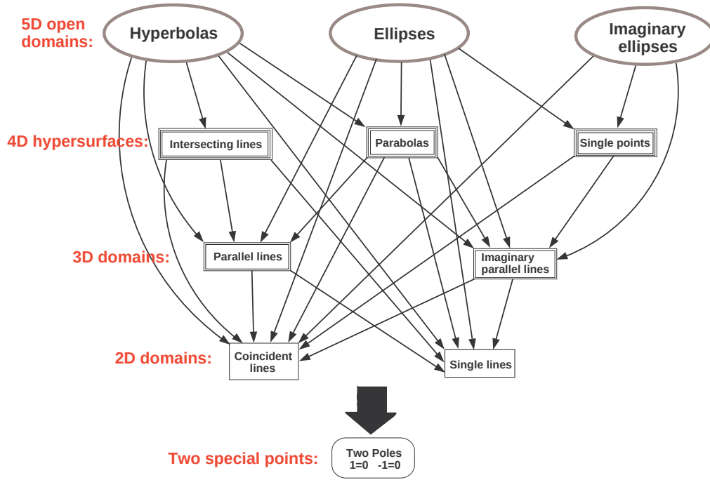
Figure 7: All the subdomains in the parameter space \mathbb{S}^5 .
