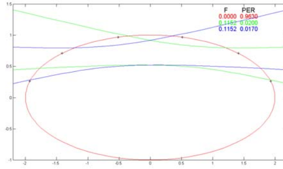
Figure 15: One global minimum (red ellipse) and two local minima (blue and green hyperbolas).
