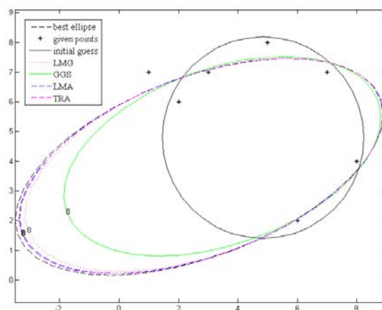
Figure 20: Progress after 8 iterations.
