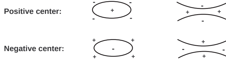
Figure 3: Conics with positive and negative centers.
