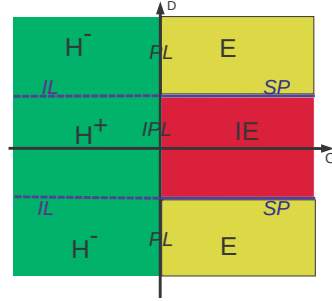
Figure 11: The CD plane for Example (4) and respective conic types.
