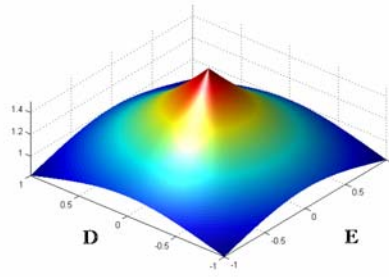
Figure 9: Graph of the objective function in Example (3).
