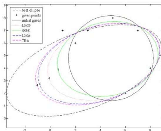
Figure 19: Progress after 4 iterations.
