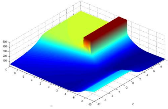
Figure 12: Graph of the objective function for Example (4).
