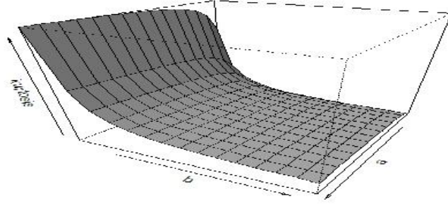
Fig.6. Variation of kurtosis, a = 1, 2, \dots, 15 and b = .1, .45, .8, \dots, 5 , for fixed \alpha=2, \beta=2.5, \theta=2.5
