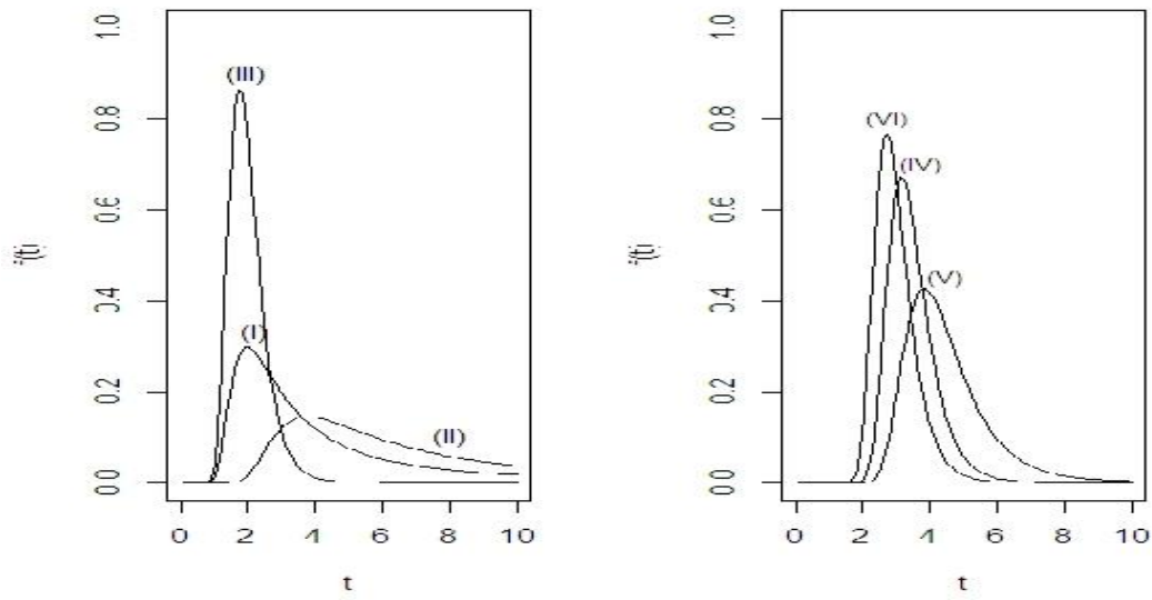
Fig.1. Plots of the BGIW density function. \alpha=2, \beta=2.5, \theta=2.5 , (I): a=0.5, b=0.5 , (II): a=2, b=0.5 . (III): a=0.5, b=4 . (IV): a=5, b=5 (V): a=6, b=3 (VI): a=3, b=5 .
