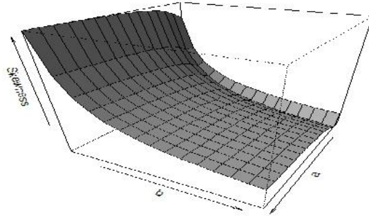
Fig.5. Variation of skewness, a = 1, 2, \dots, 15 and b = .1, .45, .8, \dots, 5 , for fixed \alpha=2, \beta=2.5, \theta=2.5
