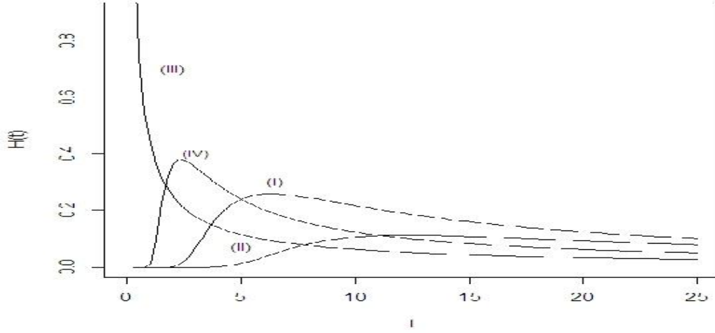
Fig.3. Plots of the BGIW hazard rate functions. (I) \alpha = 4, \beta = 2, \theta = 1.5, a = 1.5, b = 1.3 , (II) \alpha = 10, \beta = 2, \theta = 1.2, a = 1.1, b = 1.1 , (III) \alpha = 5, \beta = 0.2, \theta = 0.2, a = 12, b = 5 , (IV) \alpha = 2, \beta = 2.5, \theta = 2.5, a = 0.5, b = 0.5
