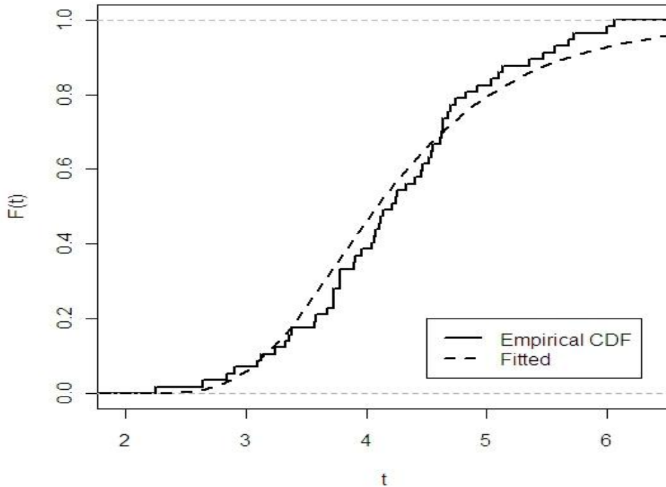
Fig. 7. Estimated cumulative function and the empirical for breaking strength of single carbon fibbers of length 1
