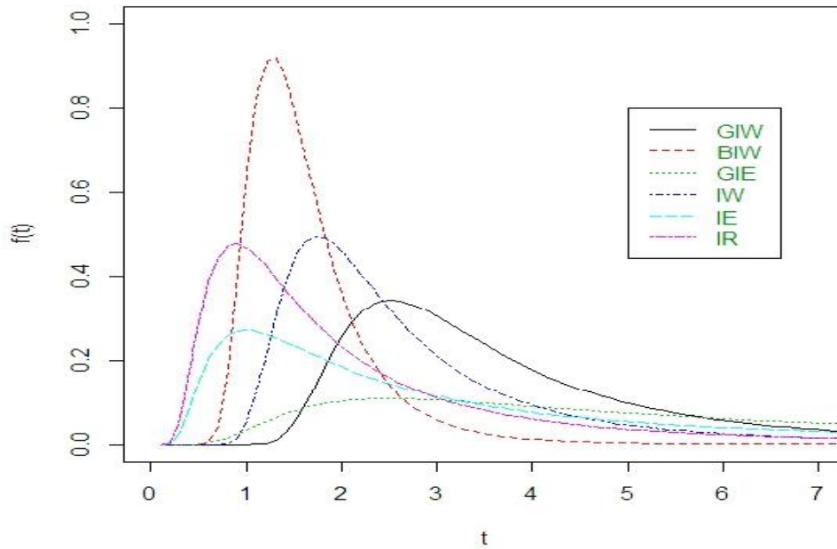
Fig.4. Plots the BGIW probability density functions of the six special models
