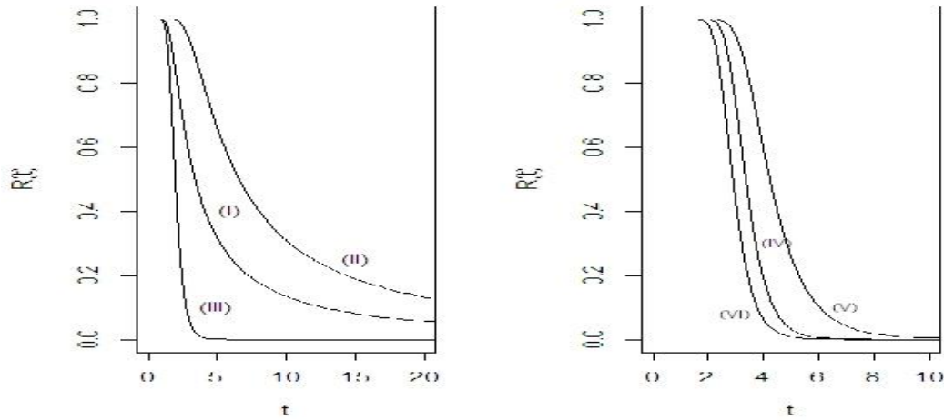
Fig.2. Plots of the BGIW reliability function. \alpha=2, \beta=2.5, \theta=2.5 , (I): a=0.5, b=0.5 , (II): a=2, b=0.5 . (III): a=0.5, b=4 . (IV): a=5, b=5 (V): a=6, b=3 (VI): a=3, b=5 .
