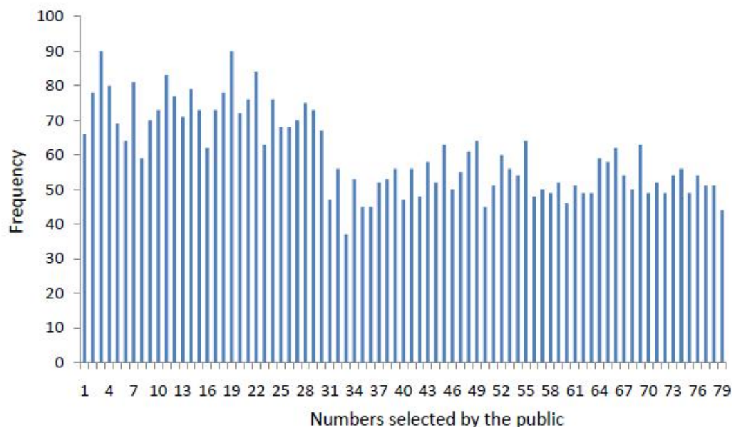
Figure 1: The number of times that each number was selected by the public on a typical day
