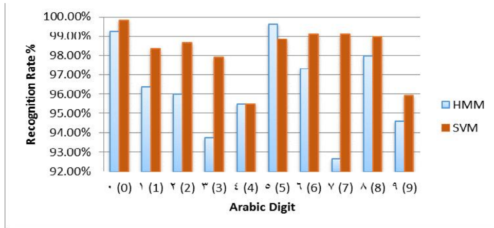
Fig. 10. Recognition rate per digit for SVM and HMM.
