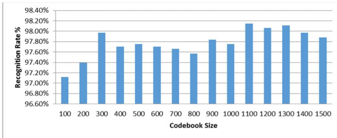
Fig. 8. Recognition rate per codebook size.
