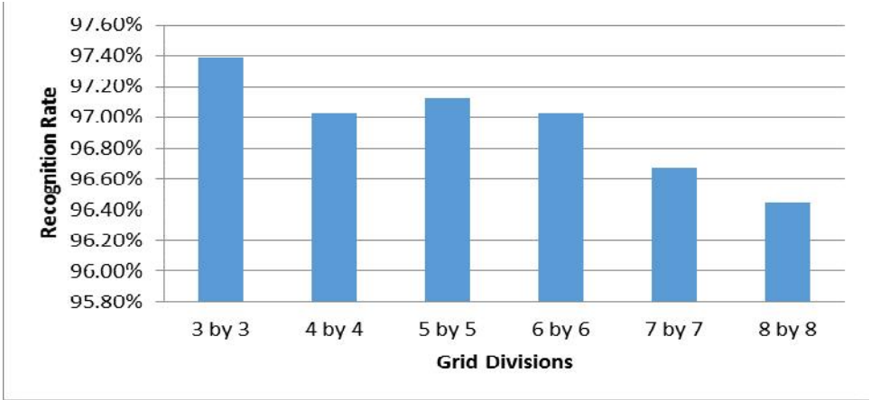
194 Fig. 7. Recognition rate at different divisions on verification data. 195
