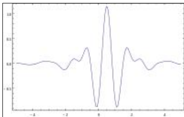
Figure 1: Wavelet example
