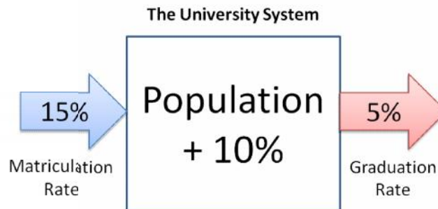
Fig. 2. University Population Growth Model
