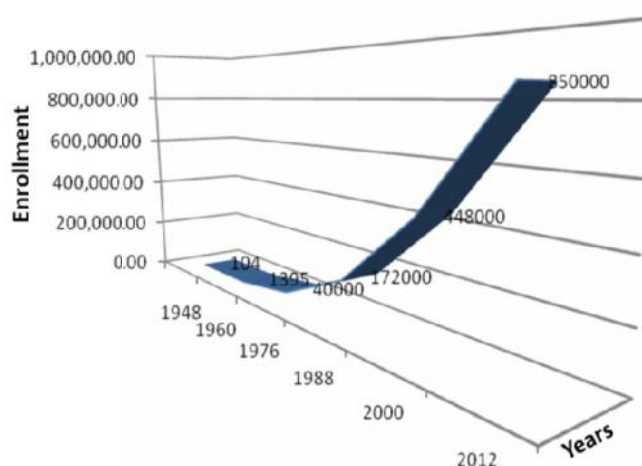
Fig. 1. Exponential growth of student enrollment in Nigerian universities
