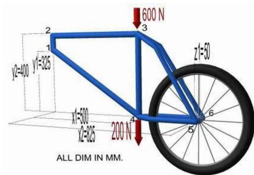
Figure 1: The Bamboo frame bicycle [8]
