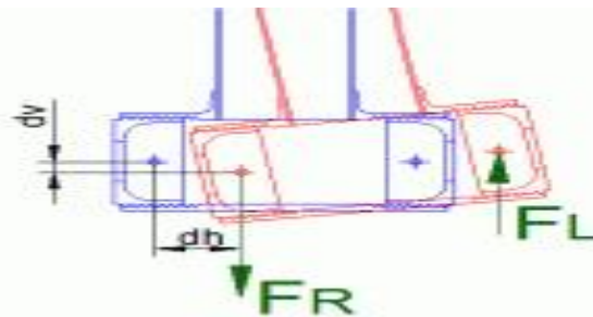
Figure: Bottom Bracket Motion while Pedaling
