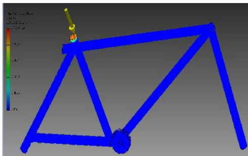
119 120 Figure 7: 1200N force simulation on the seat
