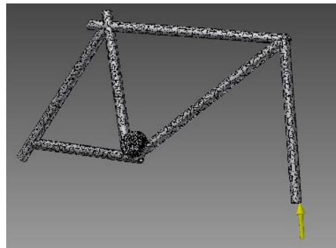
Figure: Mesh analysis of the pothole simulation
