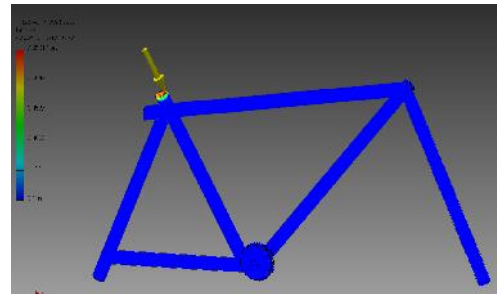
Figure 6: 600N force simulation on the seat and weight analysis
