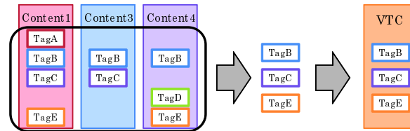
Figure 4: Figure 4. Making of a virtual typical content.
