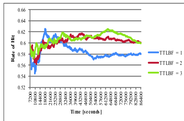
Figure 12: Hit ratios against TTL of BFs.
