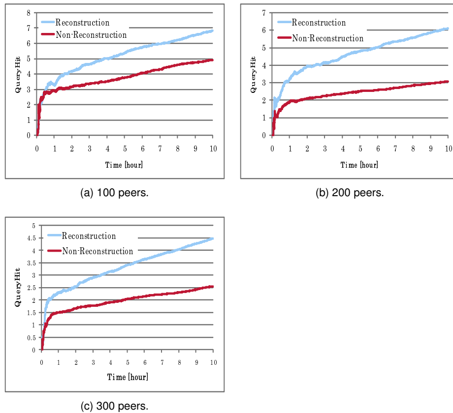
Figure 11: Averages of QueryHits.
