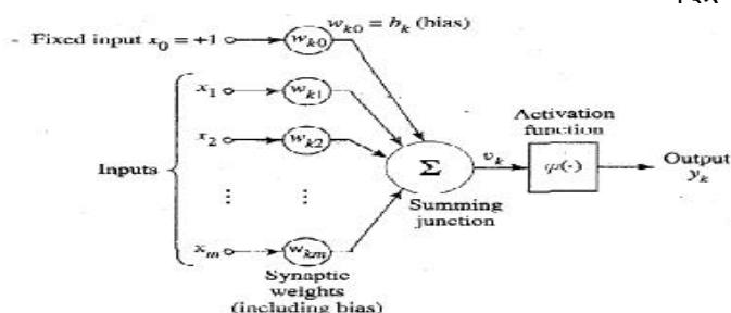
Fig. 3. A nonlinear model of a neuron w_{k0} accounts for the bias [25].
