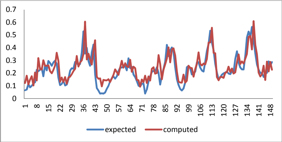
Fig. 5. A segment of the training pattern for the Hourly IN traffic with 6 lag observations at different time intervals
