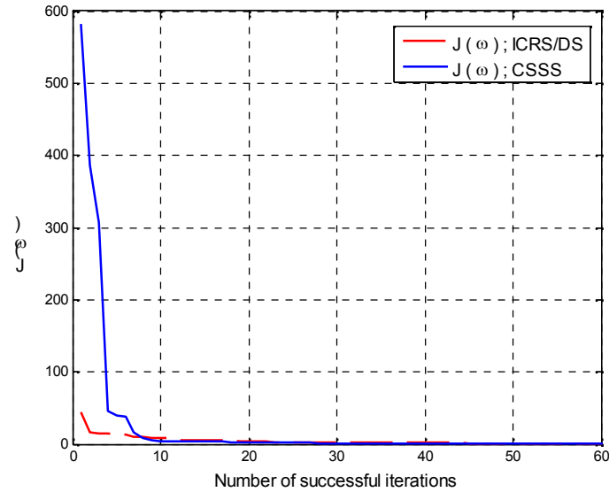
Fig.1. Plot of goal function convergence values using the CSSS and ICRS/DS algorithms. The figure axis narrowed for easy visibility – the final successful iteration number at which the goal function converges is about 150 and 900 for the ICRS/DS and CSSS, respectively.
