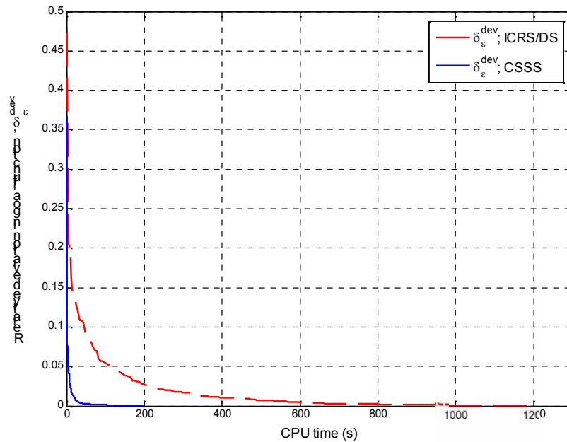
Fig. 7. Comparison of relative deviations in goal function \delta_{\epsilon}^{\text{dev}} to convergence time for the CSSS algorithm versus with the ICRS/DS algorithm for the non-linear model formalism.
