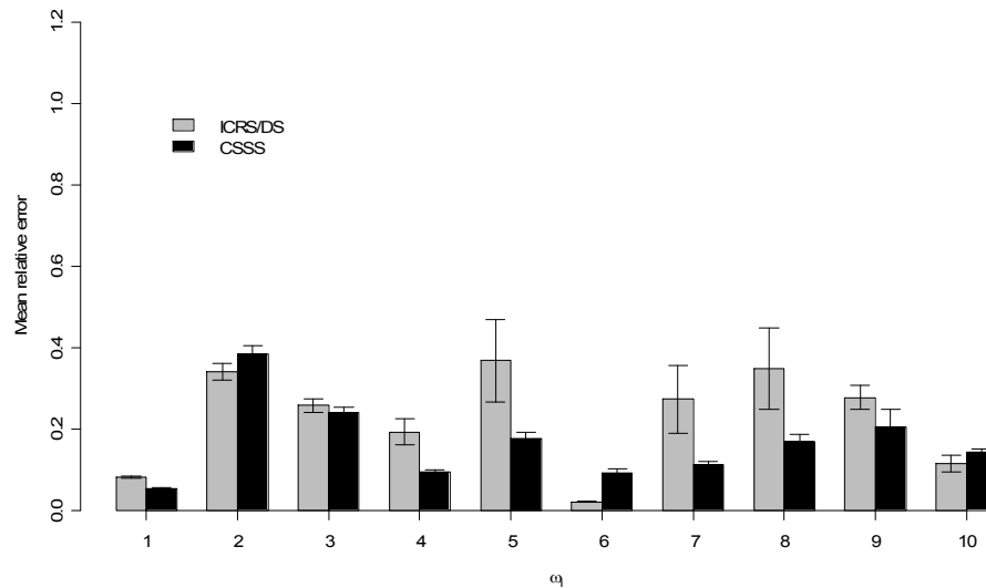
Fig. 5. Mean relative error (MRE) for the non-linear model formalism by the ICRS/DS and CSSS method, respectively. Analysis using data with a \alpha = 0.05 noise level.
