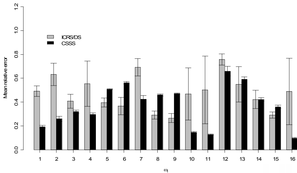
287 Fig. 2. Mean relative error (MRE) for the linear model formalism by respectively the 288 ICRS/DS and CSSS method, analysis with the noise-free dataset \alpha = 0.0 .
