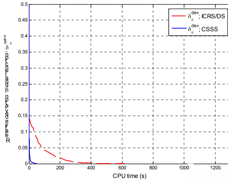
Fig. 6. Comparison of relative deviations in goal functions \delta_{\epsilon}^{\text{dev}} to convergence time for the CSSS algorithm versus with the ICRS/DS algorithm for the linear model formalism.
