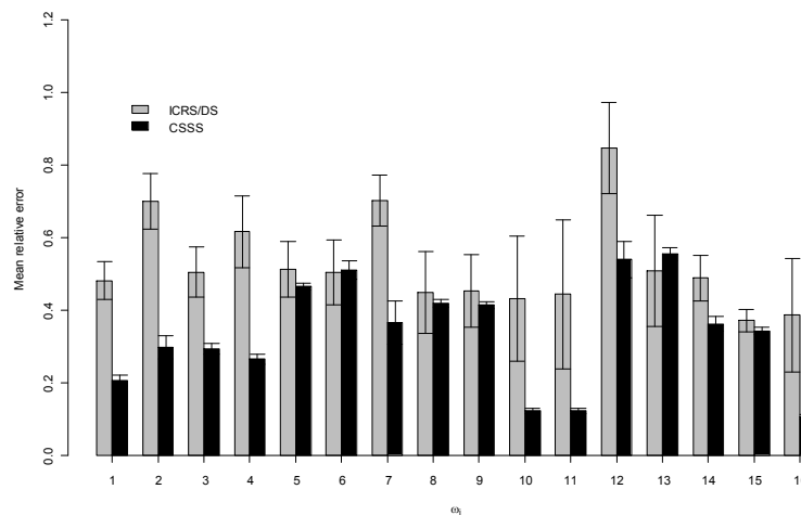
Fig. 3. Mean relative error (MRE) for the linear model formalism by the ICRS/DS and CSSS method, respectively. Analysis was done using data with \alpha = 0.05 .
