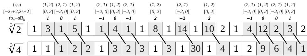
Figure 1: Continued fraction ladder of (\sqrt[3]{2}, \sqrt[3]{4})
