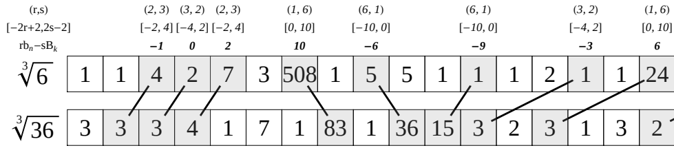
Figure 2: Continued fraction ladder of (\sqrt[3]{6}, \sqrt[3]{36})
