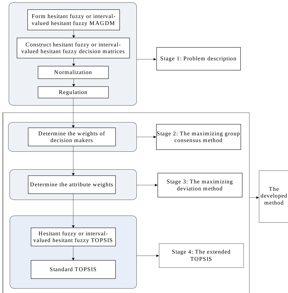
Fig. 1. The flowchart of the developed methods.
