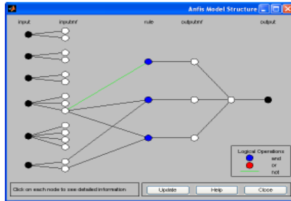
Figure 8: Shows the Structure of the j48 rules based neuro /fuzzy model
