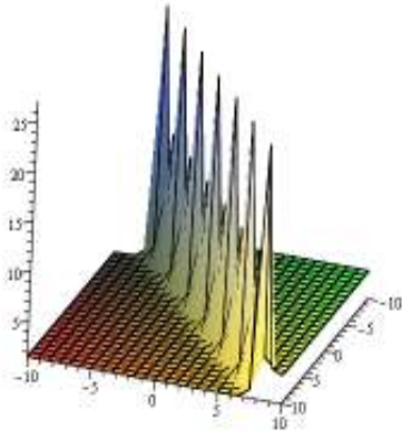
Fig. 3: Singular soliton solution u_3(\xi) when \beta=1 , k=2 , \mu=0 , \lambda=2 , E=1 and -10 \leq x, t \leq 10 .
