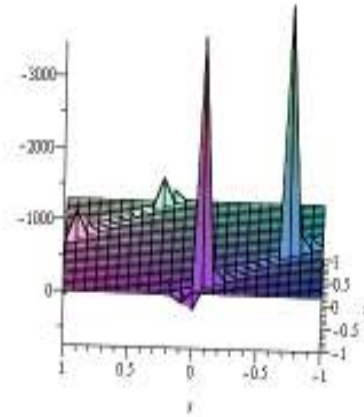
Fig. 1: Kink wave solution u_1(\xi) when \beta=1 , k=2 , \mu=1 , \lambda=3 , E=1 and -10 \leq x, t \leq 10 . Fig. 2: Periodic solution u_2(\xi) when \beta=1 , k=2 , \mu=3 , \lambda=1 , E=1 and -1 \leq x, t \leq 1 .
