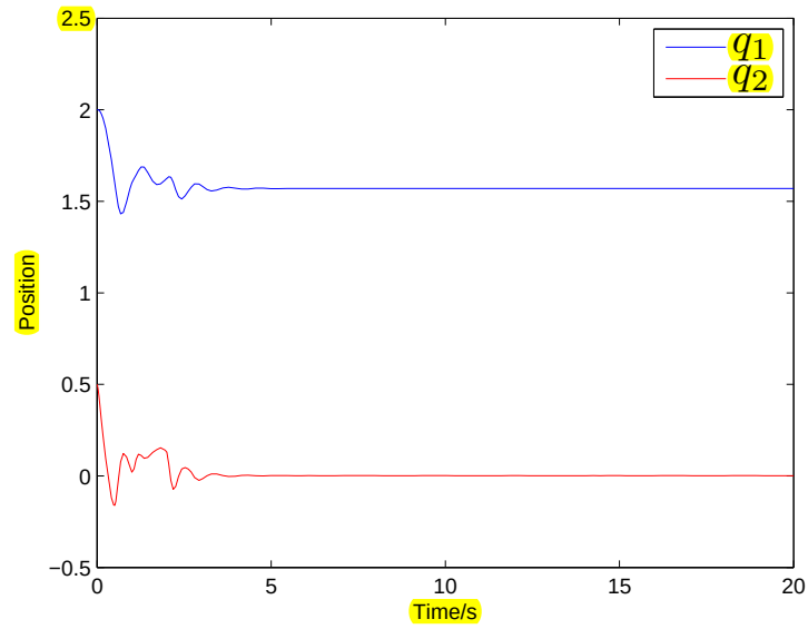
Figure 5: Response of q under time delay h = 0.5s .
