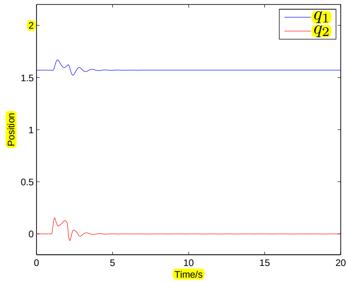
Figure 2: Response of q under time delay h = 0.5s .
