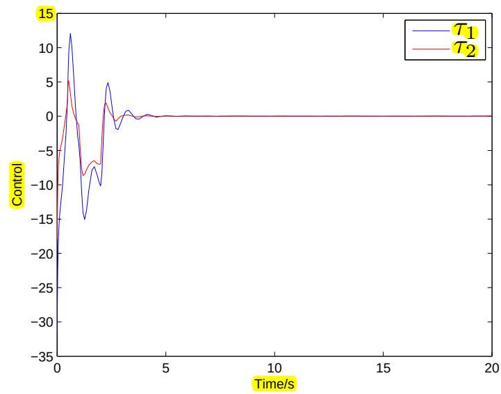
Figure 6: Control \tau under time delay h = 0.5s .
