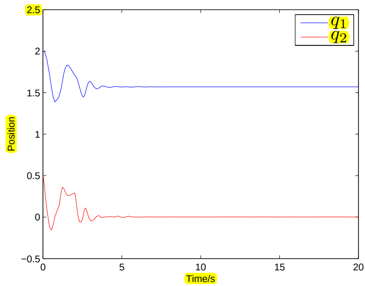
Figure 8: Response of q under time delay h = 2.5s .
