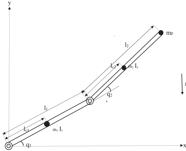
Figure 1: Planar two-link manipulator with payload.
