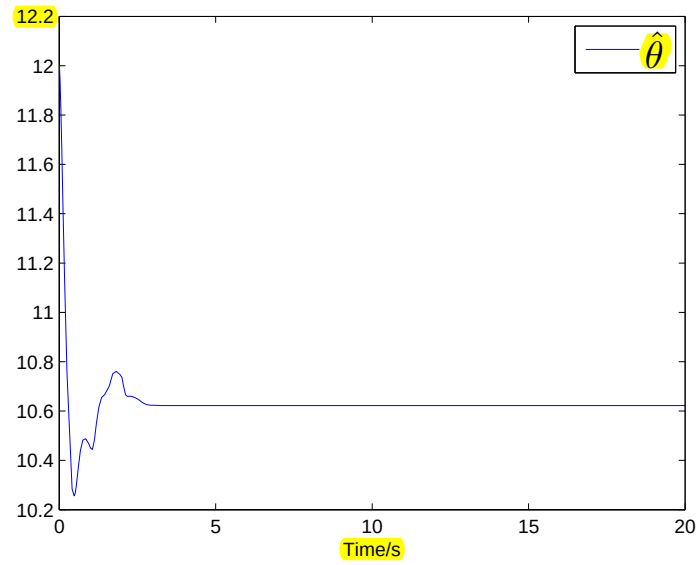
Figure 7: Estimate \hat{\theta} under time delay h = 0.5s .
