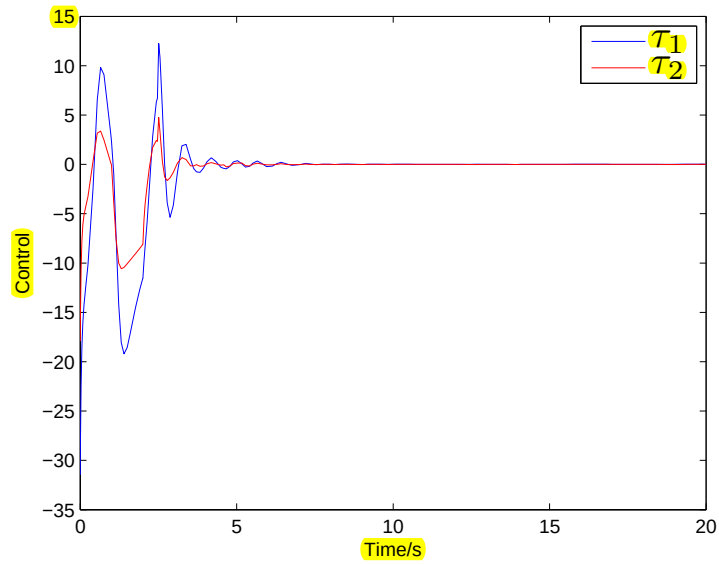
Figure 9: Control \tau under time delay h = 2.5s .
