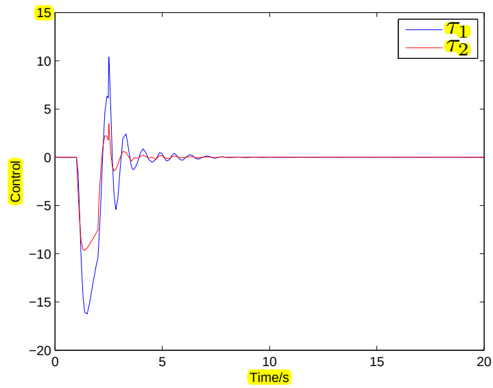
Figure 3: Control \tau under time delay h = 0.5s .
