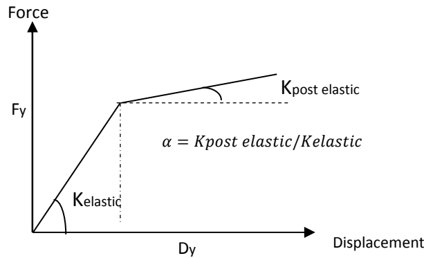
Figure 3: Base-isolation stiffness modeling.
