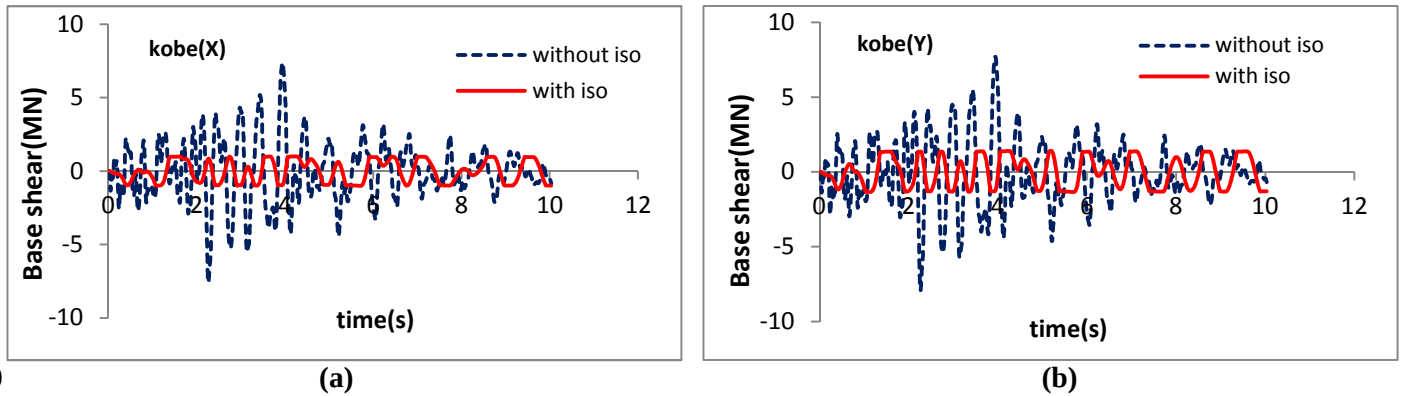
Figure 10: Time variation of base shear quantities of isolated and non-isolated tank under sanfernando, Northridge and Kobe earthquakes. a) X direction b) Y direction
