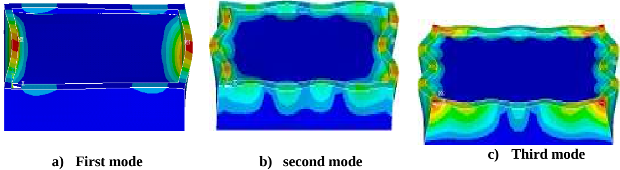
Figure 7: Displacement vector summation (X, Y, Z) for impulsive modes, a) first mode b) second mode c) Third mode
