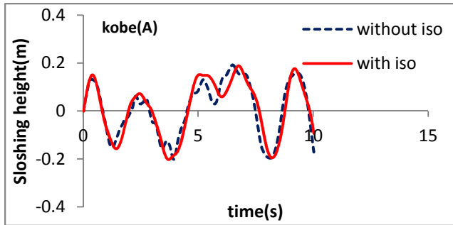
Figure 9: Time variation of sloshing quantities of isolated and non-isolated tank under sanfernando, Northridge and Kobe earthquakes. a) A location b) B location
