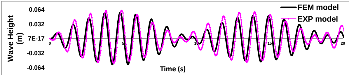
Figure 4: Comparison between FEM results of sloshing wave height and experimental measurements (P-value=0. 619>0.05).
