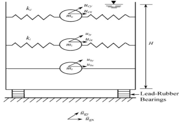
Figure 1: Structural model of base-isolated liquid storage tank.[13]
