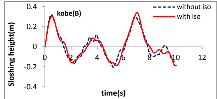
Figure 9: Time variation of sloshing quantities of isolated and non-isolated tank under sanfernando, Northridge and Kobe earthquakes. a) A location b) B location
