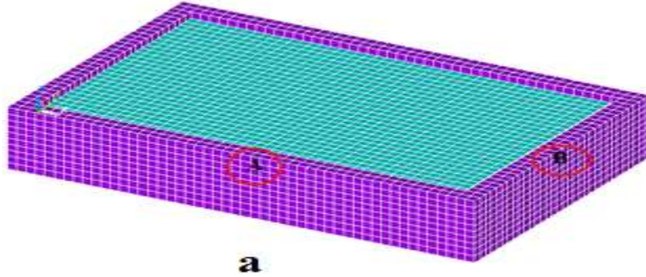
Figure 8: Finite element model of a three-dimensional rectangular tank: (a) shallow tank model
