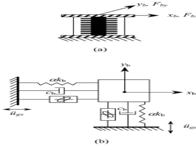
Figure 2: The isolation system. (a) Lead-rubber bearing and (b). [13]
