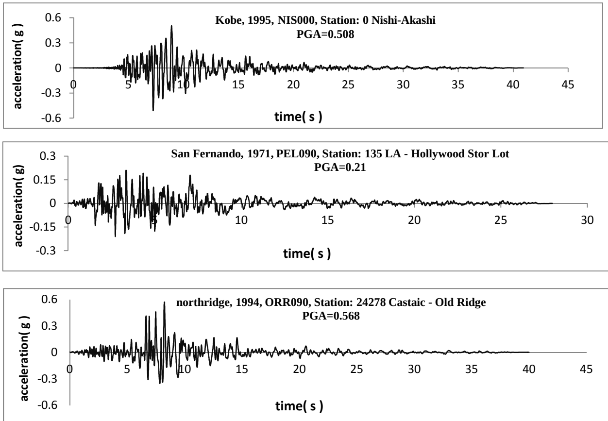
Figure 5: Time history earthquake records under x and y directions. [17]
