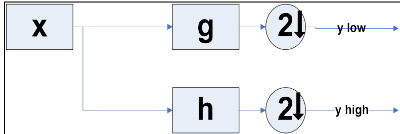
Figure 2: The multiscale decomposition analysis with DTW
