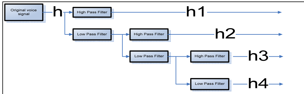
Figure 5: the 4 produced sub signals from the original voice signal by choosing n=3 .
