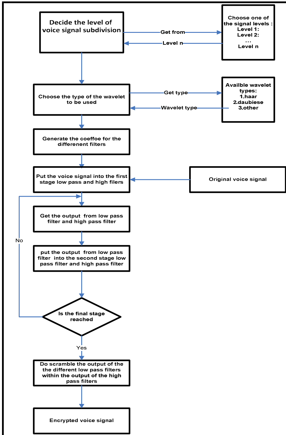
151 Figure 3: The proposed voice encryption method.
