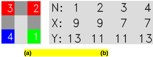
Fig. 17 Initial block of four vertices
