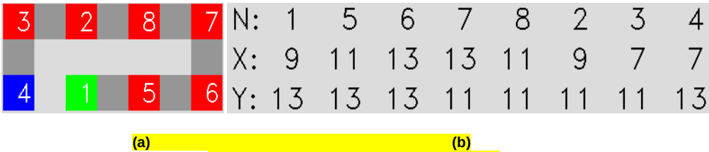
Fig. 18 Second stage of path construction
