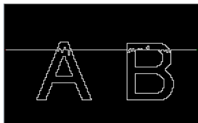
Fig. 12. Early stage of solution path construction for 'AB'
