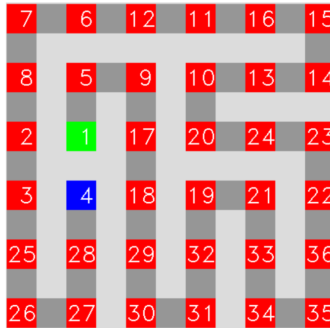
Fig. 22 Hamiltonian path: the initial block direction is left ( h=2 ), msx=5 , msy=7 , initial (x1, y1) = (7, 7) , vertex 7 is at (3,3) and vertex 35 is at (13,13)
