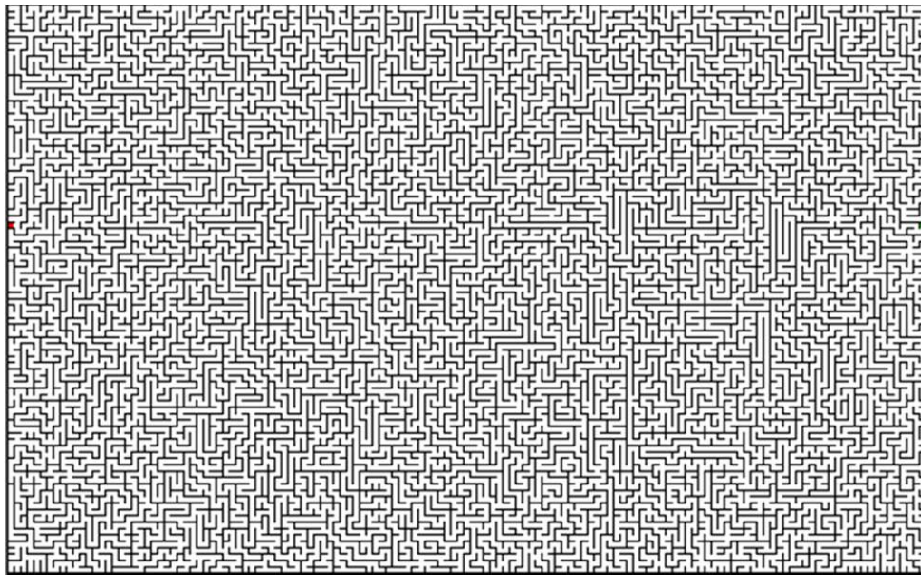
Fig. 15. Final maze for 'AB'
