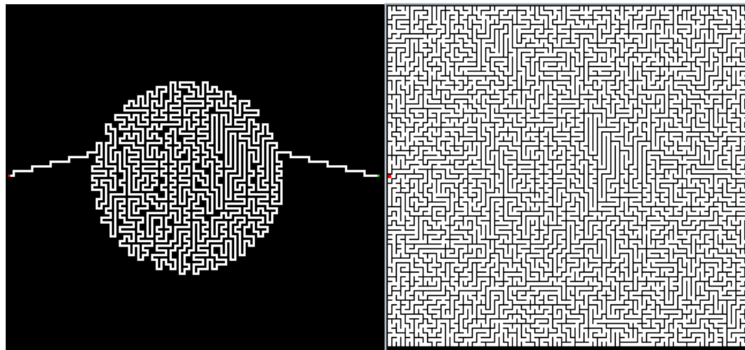
(a) (b) Fig. 23 Maze with a circle (a) Parts of solution path are straight (b) The lines are not noticeably seen
