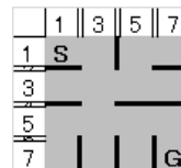
Fig. 2 Maze to be presented to a player
