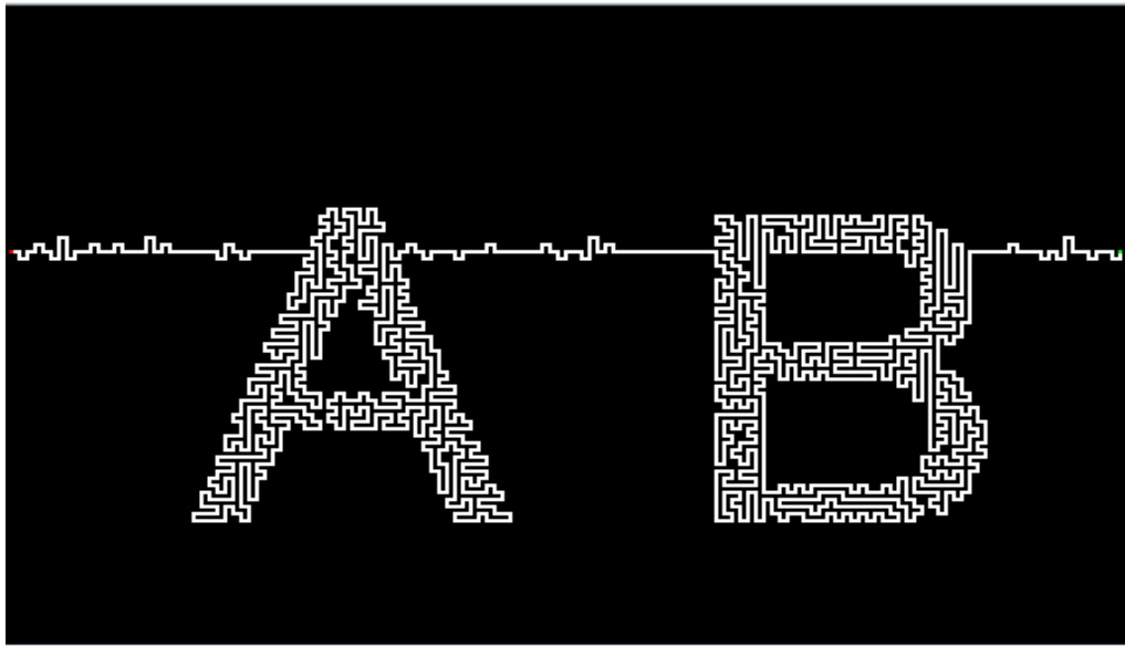
Fig. 14. Final solution path with zigzag for 'AB'
