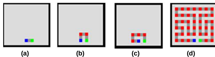
Fig. 9 Construction of block spanning tree with the block of two vertices and the Hamiltonian path
