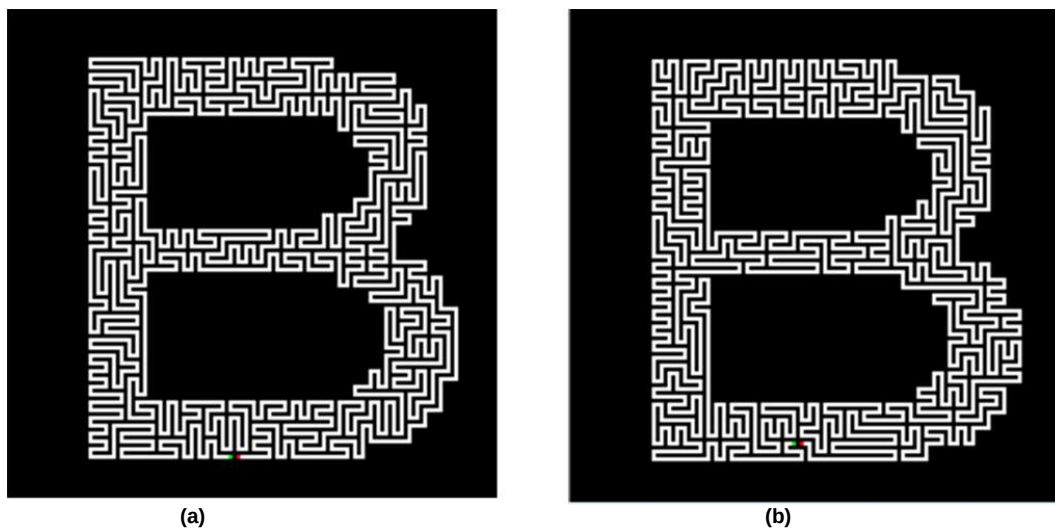
Fig. 7 (a) Block Hamiltonian path with the start and goal at the bottom; and (b) block Hamiltonian path with the start and goal in the middle of the picture.
