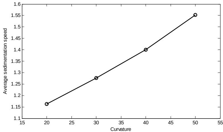
368 Fig. 12 Average sedimentation speed as a function of curvature.
