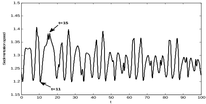
Fig. 8 Sedimentation speed of one fiber.
