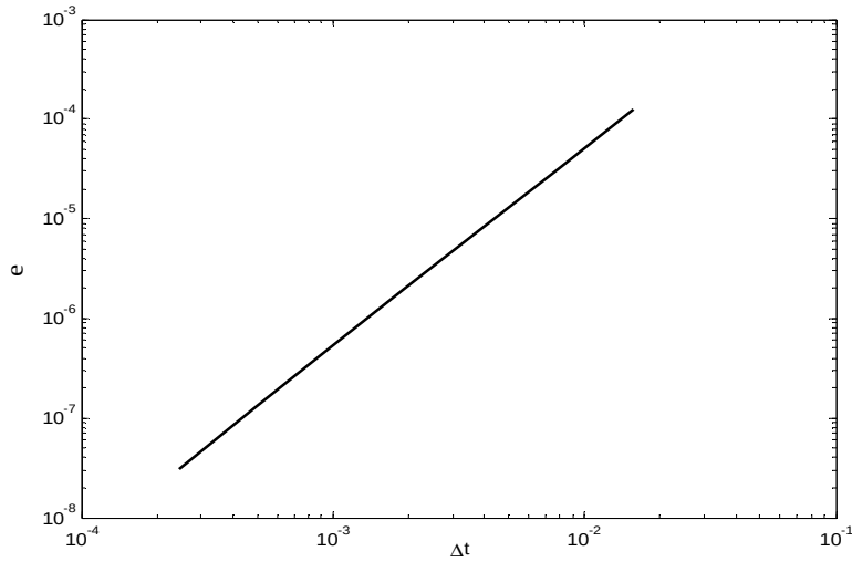
263 Fig. 1 loglog plot of the error in fiber position plotted as a function of \Delta t at the end time t = 1 . In this case 264 \Delta s = \frac{1}{64} . 265
