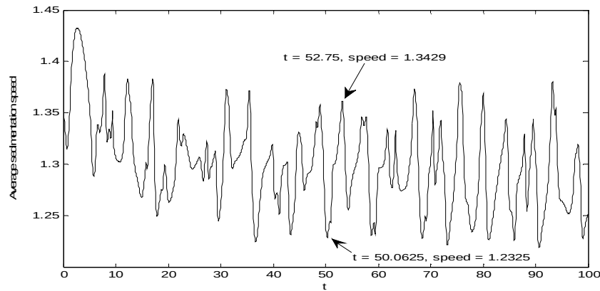
Fig. 16 Average sedimentation speed as a function of time for 2 fibers with a vertical distribution.
