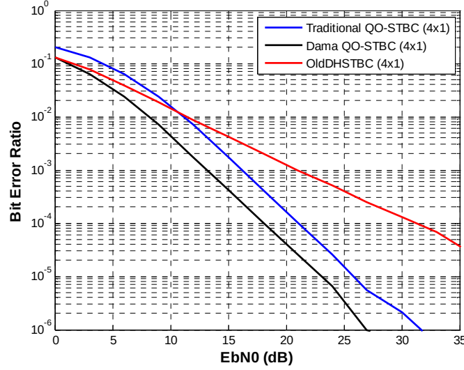
Figure 1: Comparison of traditional QO-STBC, Interference-free QO-STBC and Dama-DHSTBC for 4 x 1 MISO System
