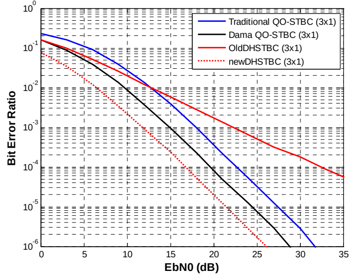
Figure 3: Comparison of new QO-STBC with traditional QO-STBC (3x1)
