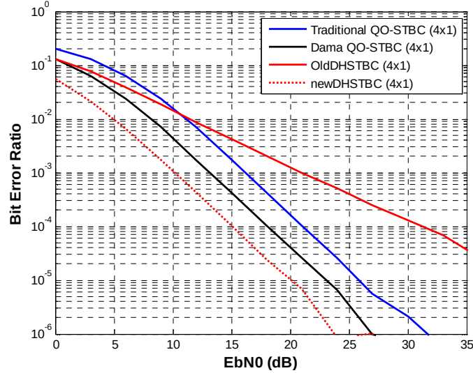
Figure 2: Comparison of new QO-STBC with traditional QO-STBC (4x1)
