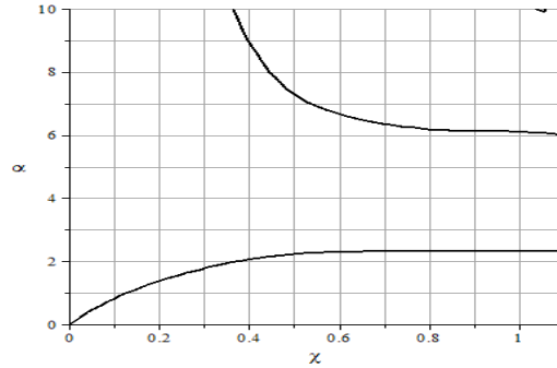
173 174 175 Fig. 3. Plot of \alpha as a function of \chi of the relation v_7(1, \chi, \alpha) = 0
