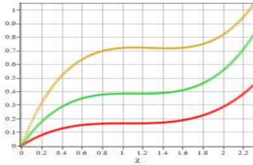
Fig. 1. \chi curves of v_3(z, \chi) at z = 0.4, 0.6, 0.8
