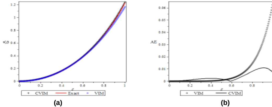
148 149 150 Fig. 2. A comparison between standard VIM and CVIM results, (a) solutions and (b) 151 absolute error 152
