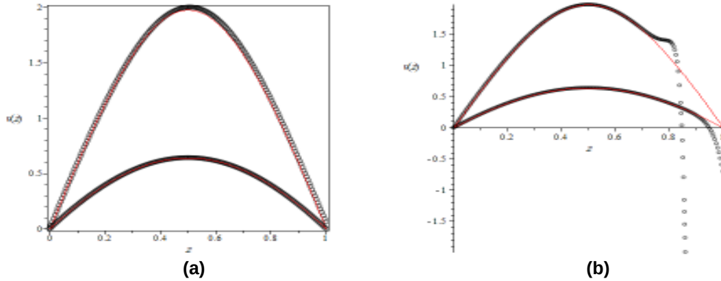
Fig. 5. A comparison between CVIM and VIM solutions (points) along with the exact solutions (lines), (a) CVIM results and (b) standard VIM results
