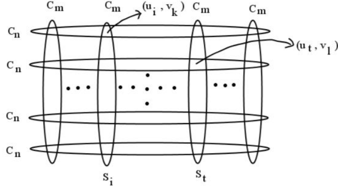
FIGURE 5. Normal product of even cycle and any cycle
