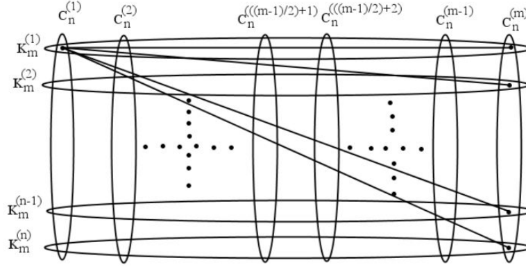
FIGURE 6. Normal product of cycle and complete graph
