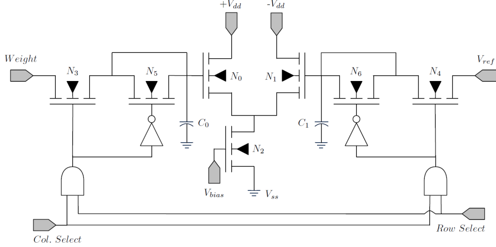
Fig. 3. Modified Synapse with Analog Memory
