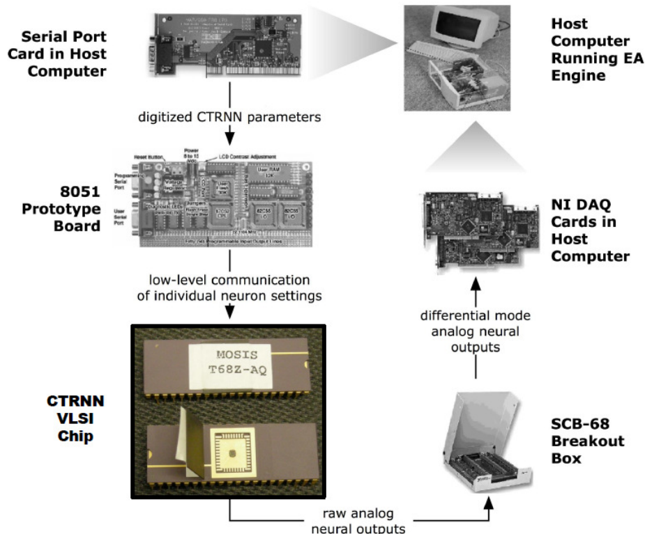
Fig. 6. A Schematic view of the Experimental Setup
