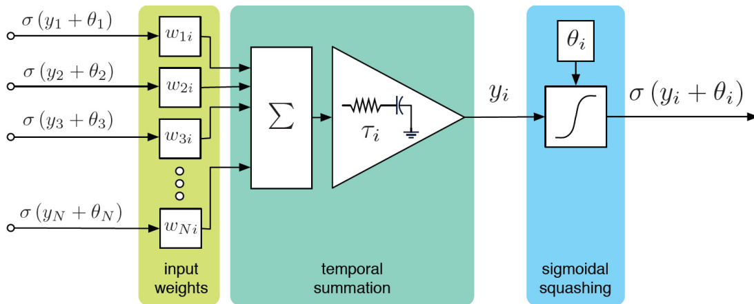
Fig. 1. Conceptual Hardware CTRNN Modules
