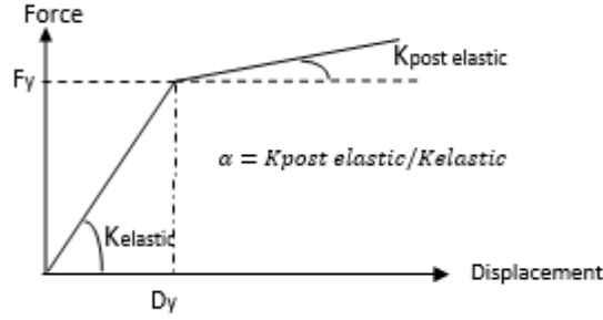
Figure 3: Base-isolation stiffness modeling.
