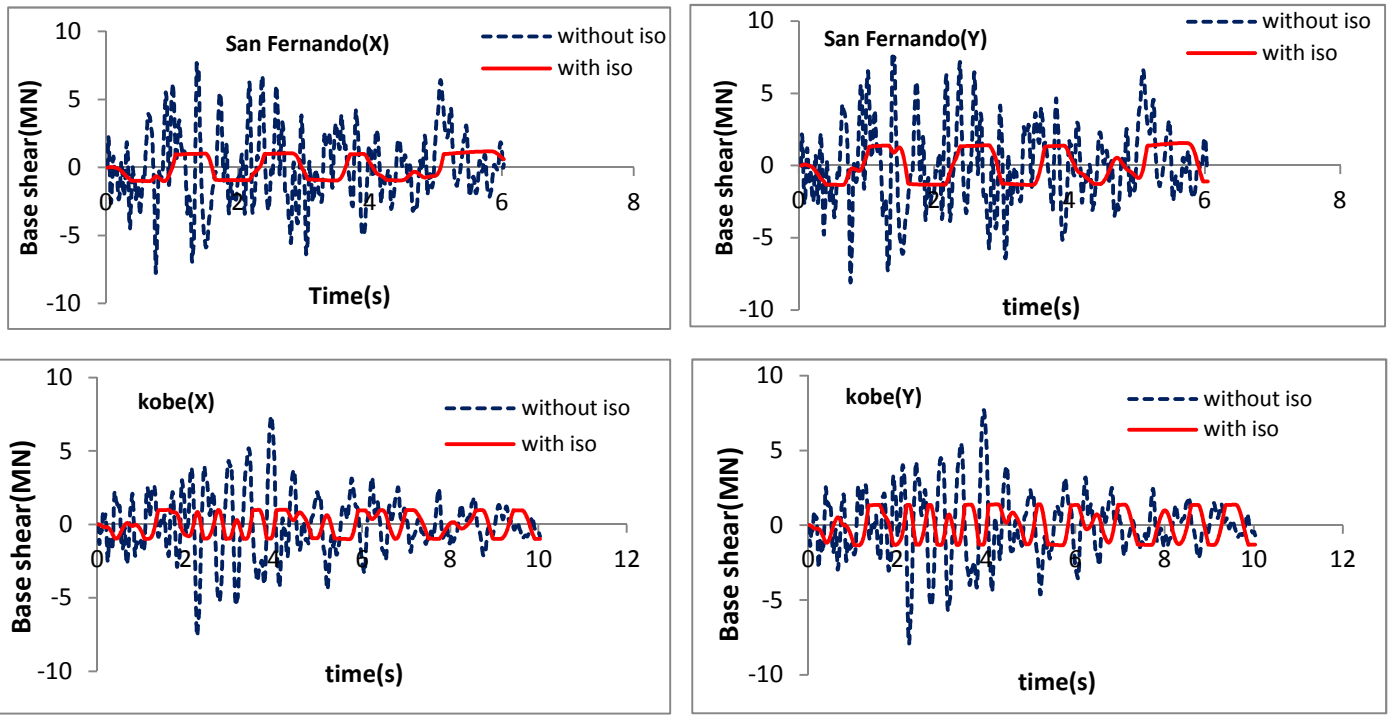
(a) (b) Figure 10: Time variation of base shear quantities of isolated and non-isolated tank under sanfernando, Northridge and Kobe earthquakes. a) X direction b) Y direction
