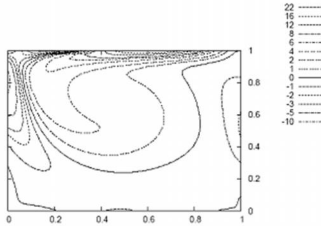
Figure:11 Constant-vorticity lines in the cavity, Re= 400
