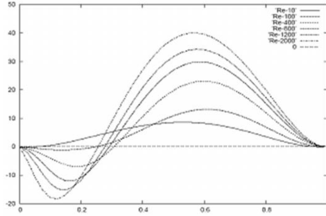
Figure:2 Distribution of upper wall vorticity for Re= 10, 100, 400, 800, 1200, 2000 .
