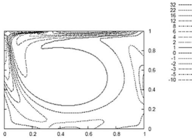
Figure:12 Constant-vorticity lines in the cavity, Re= 1200
