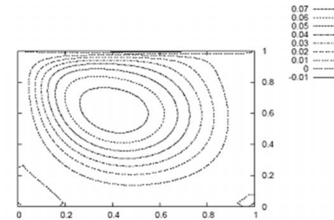
Figure:7 Streamlines for laminar flow in the cavity, Re = 400 .
