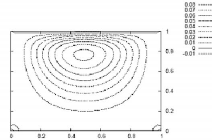
Figure:6 Streamlines for laminar flow in the cavity, Re = 10 .
