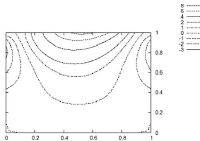
Figure:10 Constant-vorticity lines in the cavity, Re = 10
