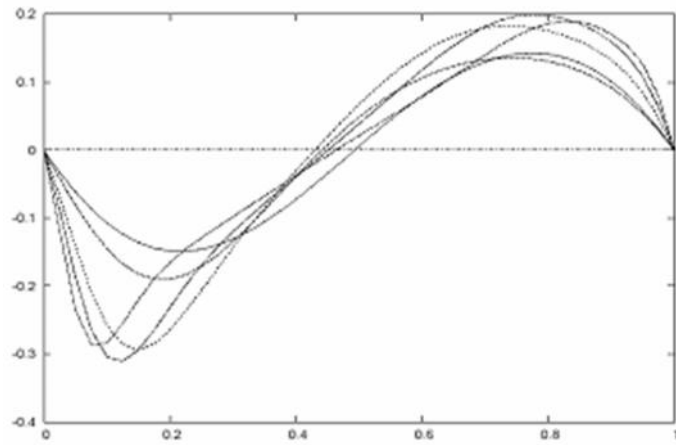
Figure:5 u-velocity on the line x=0.5 for Re= 10,100,400,800,1200,2000 .
