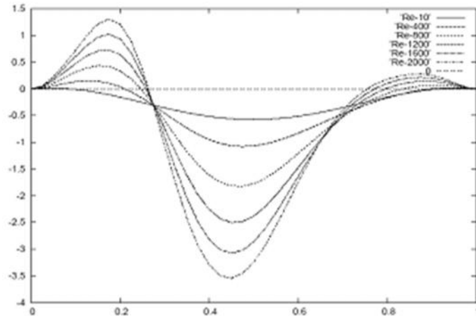
Figure:3 Distribution of lower wall vorticity for Re= 10, 100, 400, 800, 1200, 2000 .
