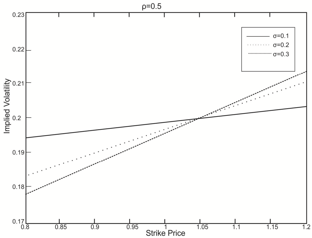
Figure 5: Implied Volatility Surface when \rho = 0.5
