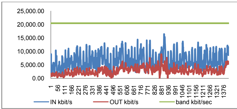
Fig. 4.A segment of Bandwidth utilization for the period January 2010 to September 2010.
