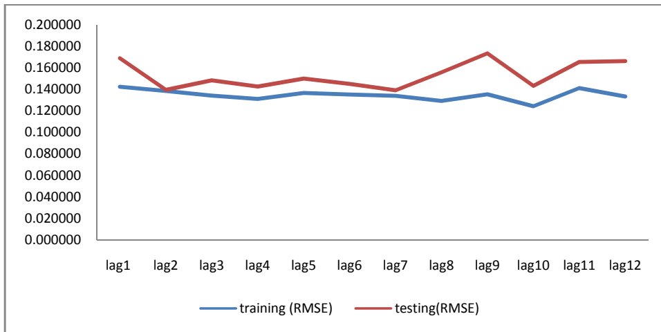
Fig. 9. The root mean square error of the training and test set of the Daily IN traffic at different lag observations
