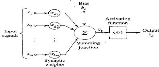
Fig. 2. Nonlinear model of a neuron [25].
