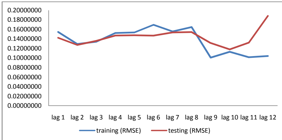
Fig. 10. The root mean square error of the training and test set of the Daily OUT traffic at different lag observations
