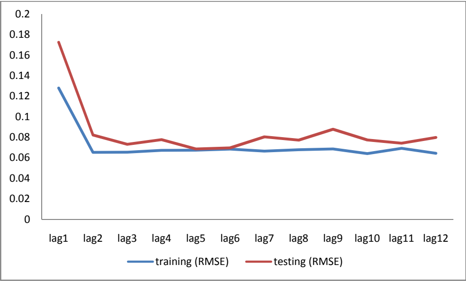
Fig. 8. The root mean square error of the training and test set of the Hourly OUT traffic at different lag observations
