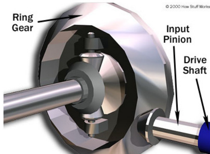
Figure 1: Hypoid bevel gears in a car differential
