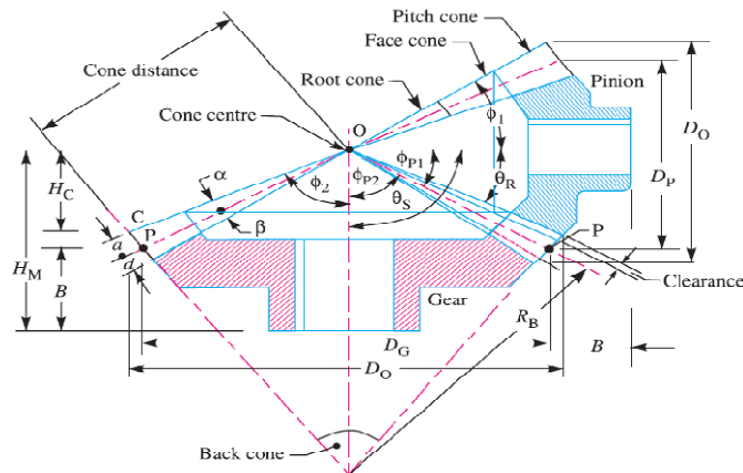
Figure 2.0: Nomenclature of a meshed bevel gear
