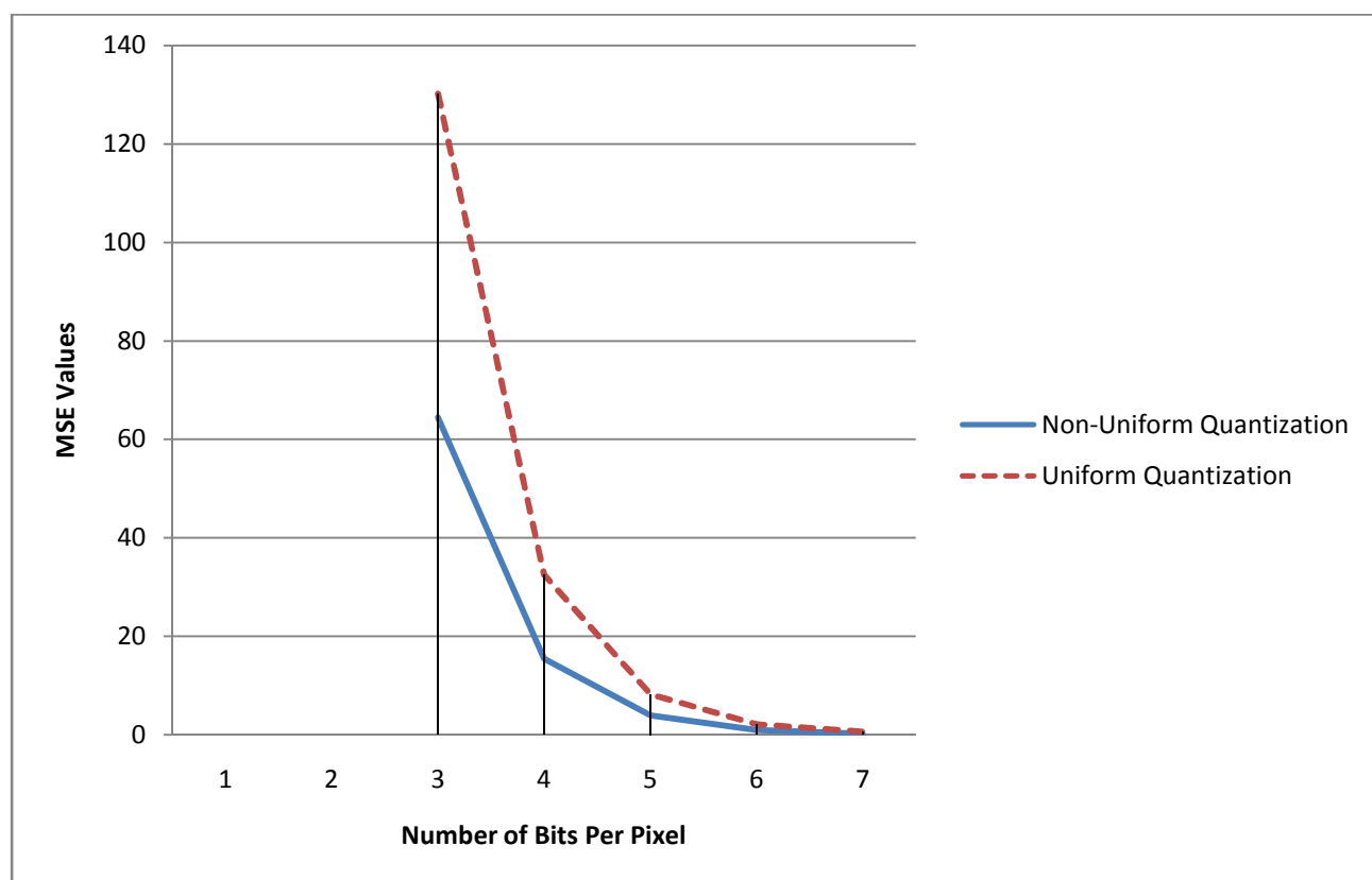
360 Figure 5.1: Plot of MSQE Values for Non-uniform and Uniform Quantization
