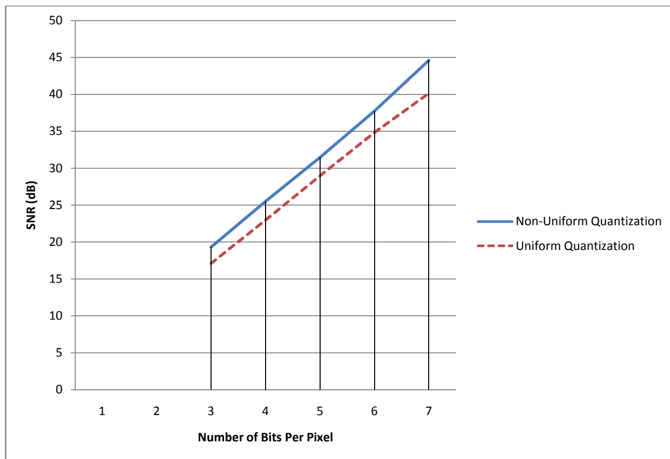
366 Figure 5.2: Plot of SQNR in decibels (dB) for Non-uniform and Uniform Quantization
