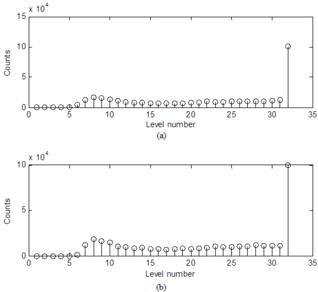
Figure 4.1: Histogram Plot of 5 bpp Quantized Fingerprint Output (a) and 8 bpp Source fingerprint Input (b)
