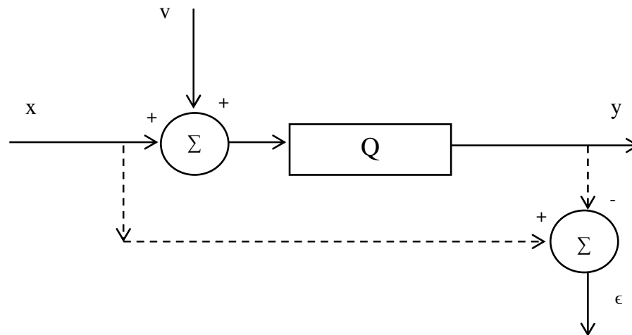
Figure 2.2: The Non-subtractive dithered quantization schematic.
