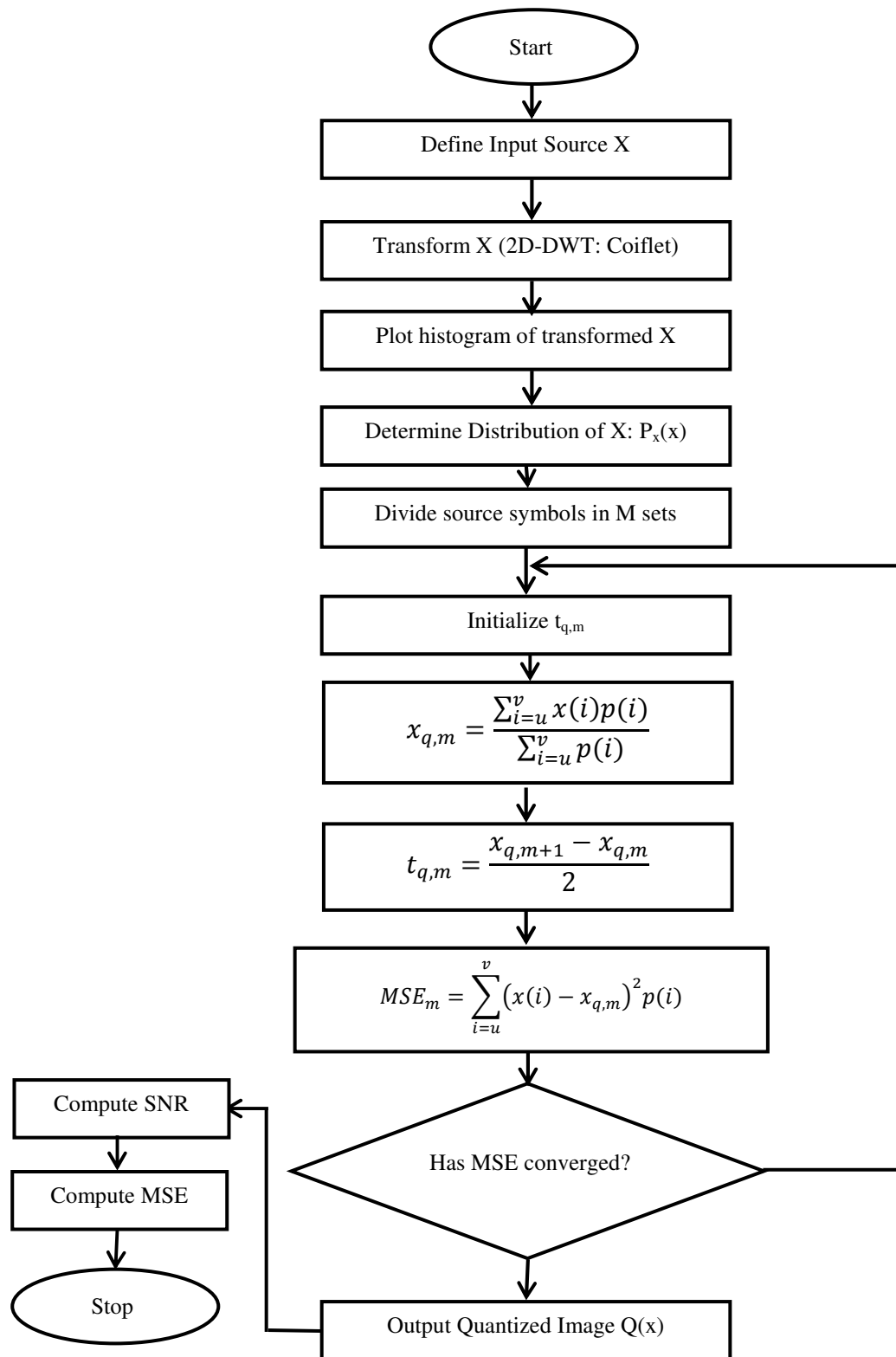
Figure 4.4: Flowchart of the Lloyd-Max Quantization Procedures
