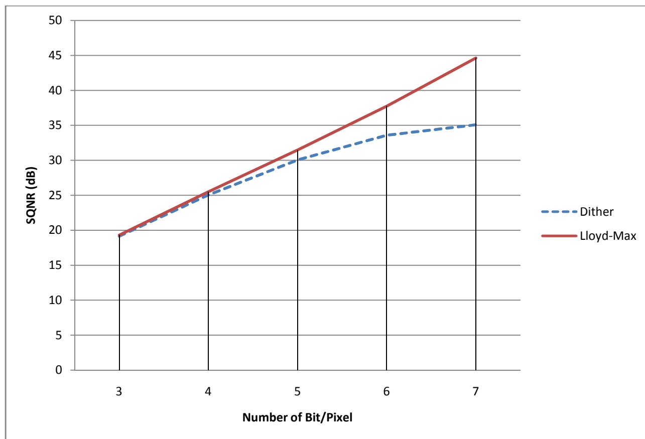
Figure 5.4: Plot of SQNR in decibels (dB) for Dither-based Non-uniform Quantization and Lloyd-Max Non-uniform Quantization Schemes
