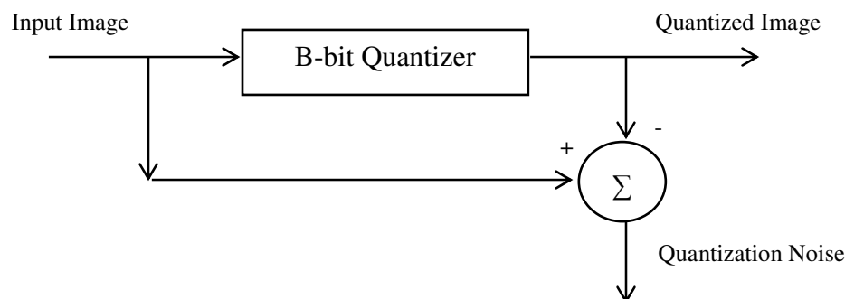
Figure 2.1: Block Diagram of Quantization Process and the Associated Noise
