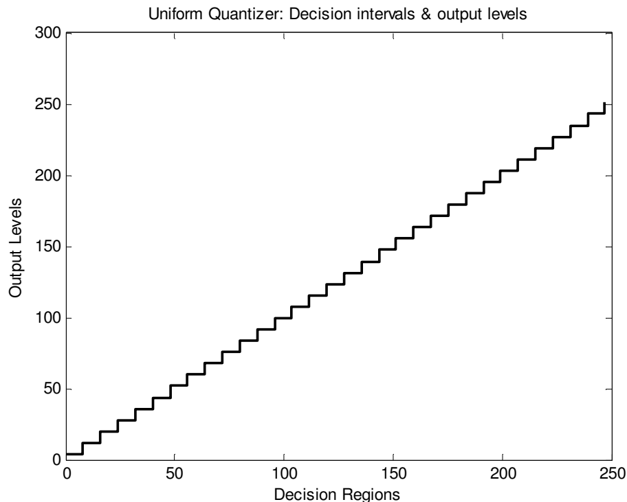
264 Figure 4.2: Plot of the Uniform Quantization Output Levels at 5 bpp
