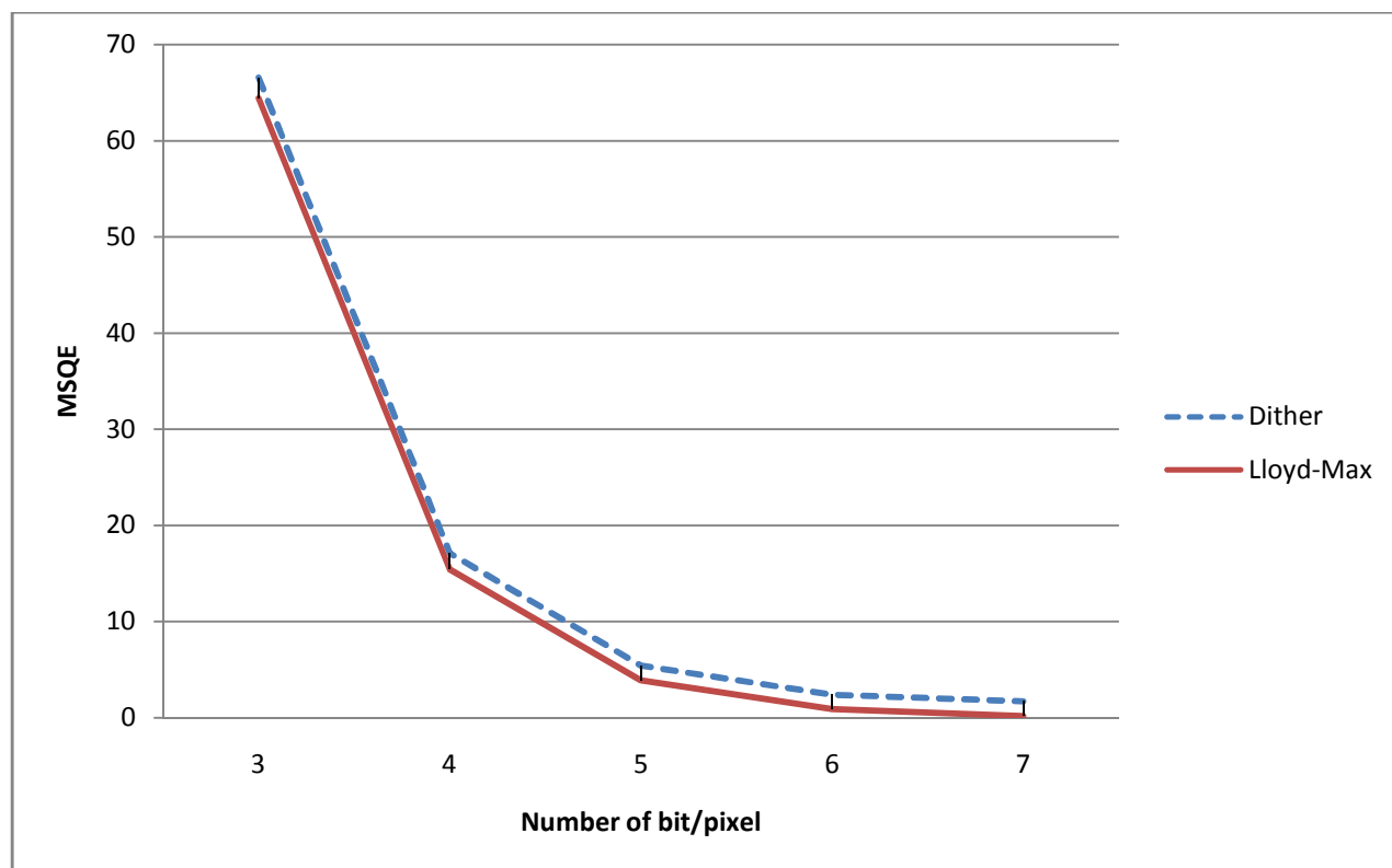
Figure 5.3: Plot of MSQE Values for Dither-based Non-uniform Quantization and Lloyd-Max Non-uniform Quantization Schemes
