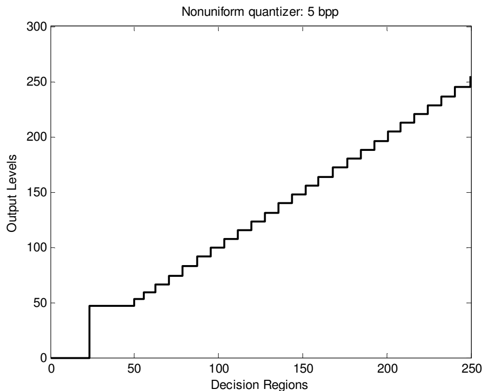
Figure 4.3: Plot of the Non-uniform Quantization Output Levels at 5 bpp
