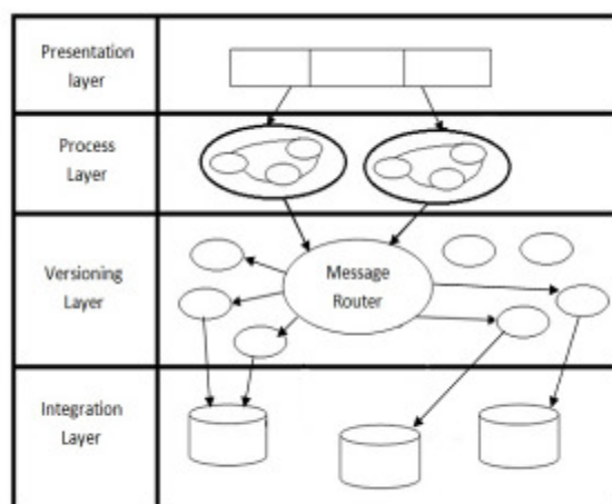
Figure -2- New Structure of SOA layers
