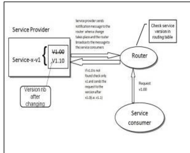
Figure 9: Non-breaking Functional change
