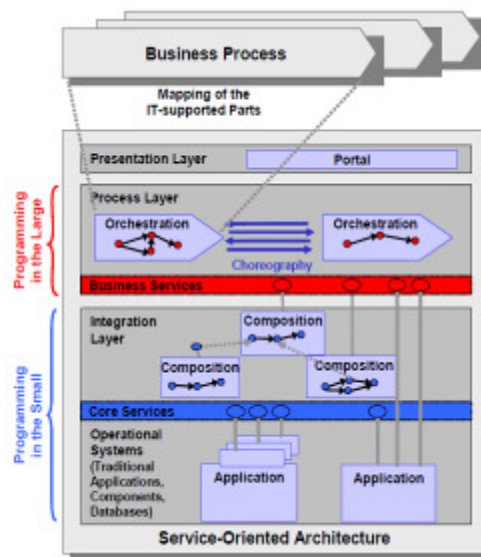
Figure-1- SOA layers
