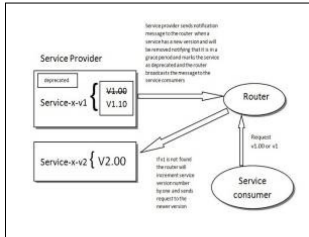
Figure 10: Breaking change
