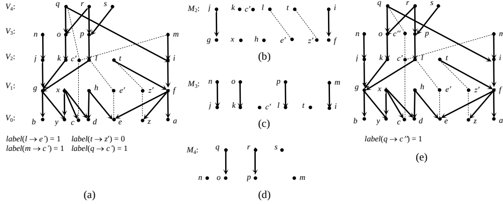
Fig. 13. Illustration for generation of virtual nodes
