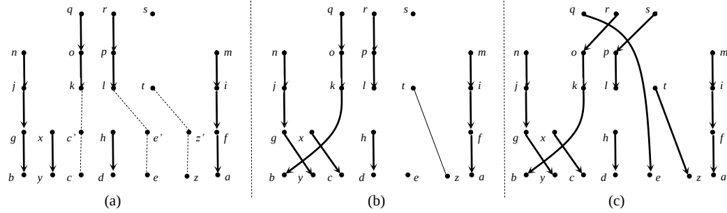
Fig. 10. Result after removing virtual nodes
