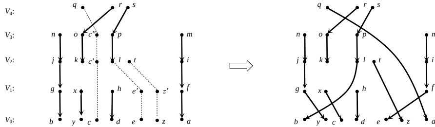
Fig. 17. Transforming the chains generated by Algorithm GenChain() to the final result
