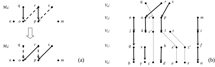
Fig. 14. Illustration for generating virtual nodes
