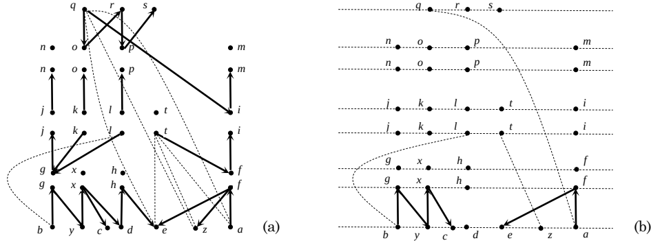
Fig. 16. Illustration for global alternating graphs and node-disjoint paths
