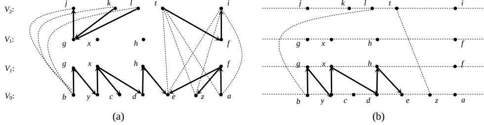
Fig. 12. Illustration for combined graphs and node-disjoint paths
