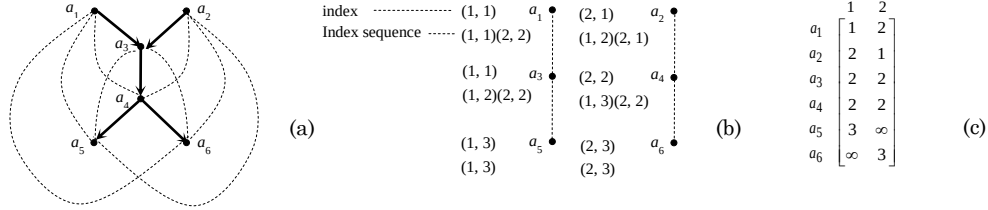
Fig. 2. Illustration for transitive closure and index
