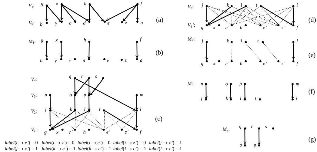
Fig. 9. Illustration for generation of chains
