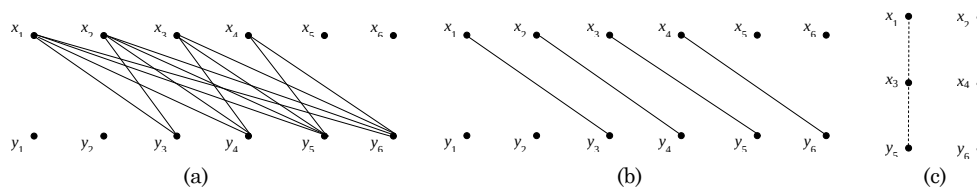
Fig. 3. Illustration for poset decomposition
