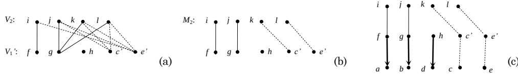
Fig. 7. Illustration for virtual nodes and chains containing virtual nodes
