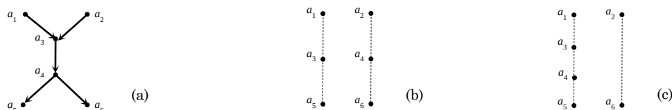
Fig. 1. Illustration for DAG decomposition
