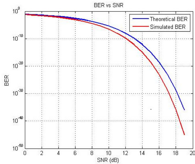
Figure3. BER of QPSK-OFDM with AWGN
