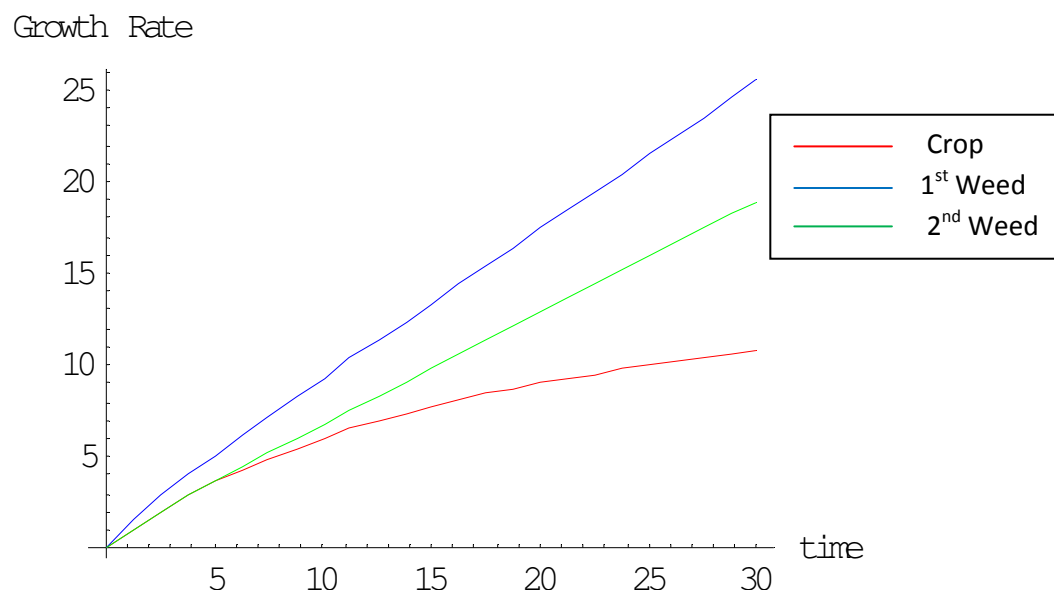
Figure 3.1 Rate of growth of Crop and Two-Species of Weed Coexistence
