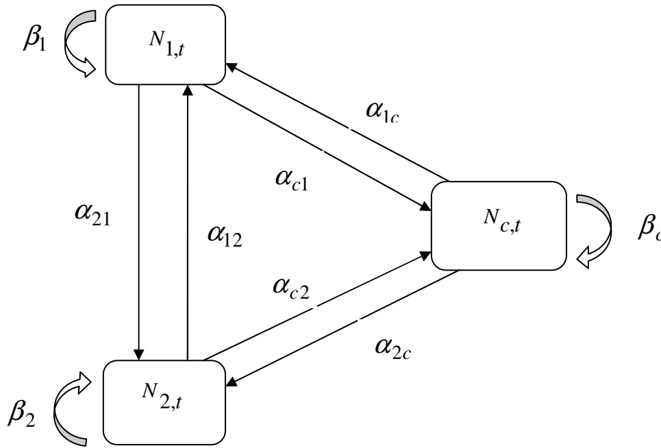
Figure 2.1 Schematic Model for Weed-Crop Competition of Homogeneous Population Density
