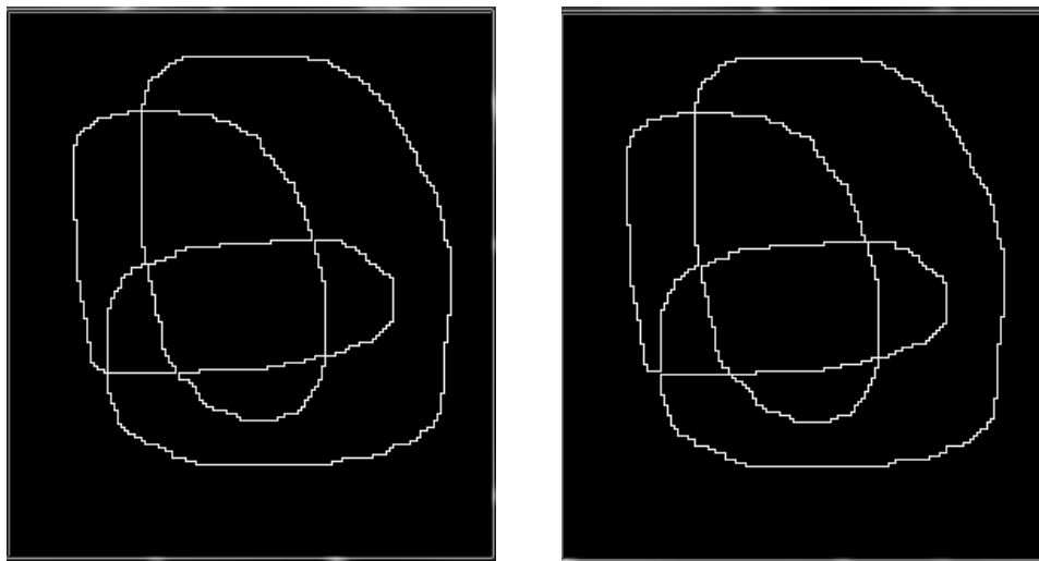
(b) Fig. 30 (a) Set of cycles partitioned, some vertices and edges overlap around some intersections: (a) partitioned X, 5 cycles; (b) partition Y, 3 cycles
