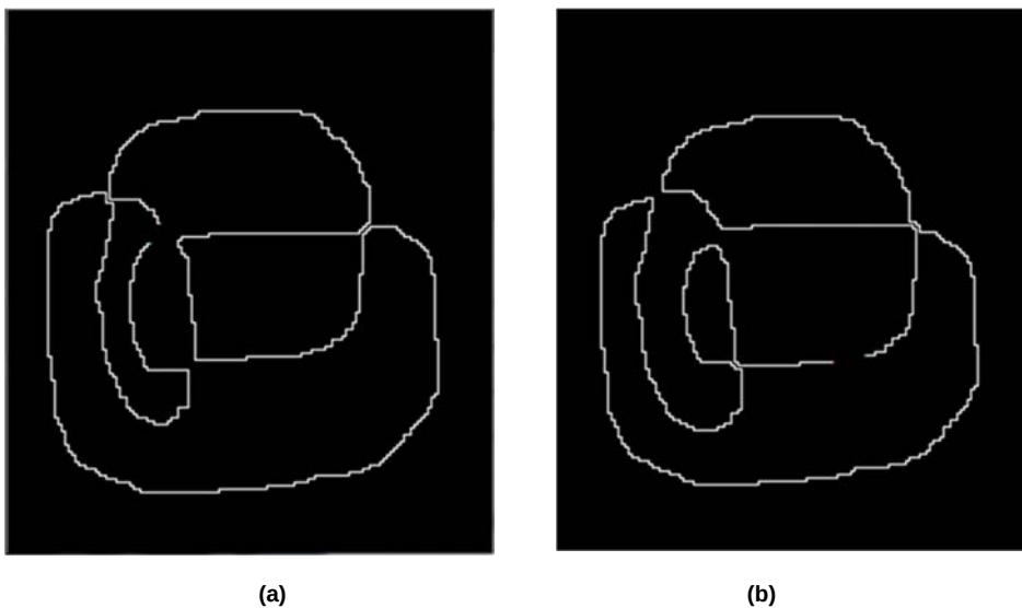
Fig. 11 Merged one single cycle: (a) X part; (b) Y part
