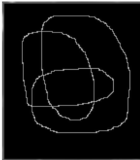
Fig. 29 Cycles are extracted (8 contour cycles), most parts overlap
