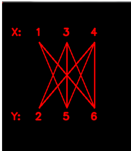
Fig. 9 Region graph bi-partitioned.
