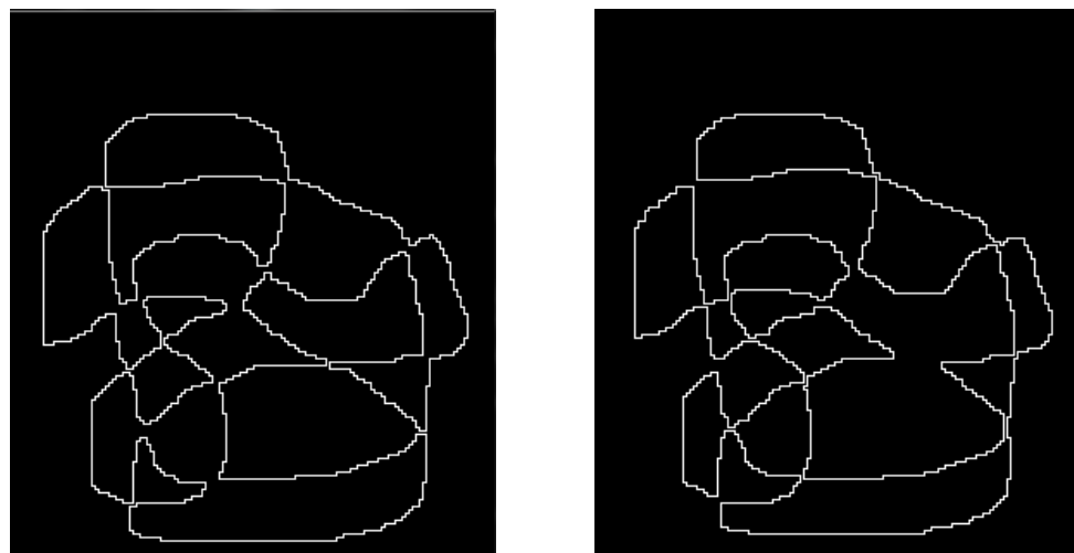
Fig. 26 Merged cycle (a) Partition X; Partition Y
