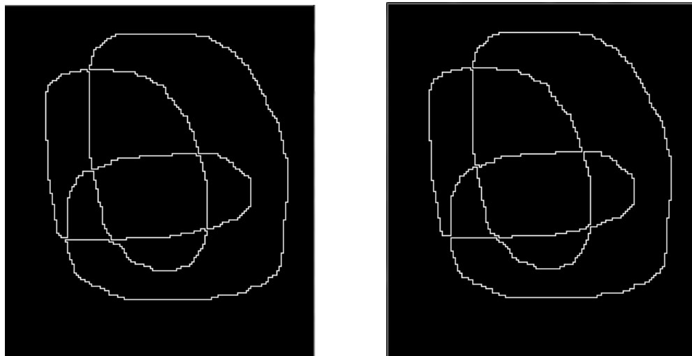
Fig. 32 cycles are merged; (a) partition X; merged; (b) partition Y
