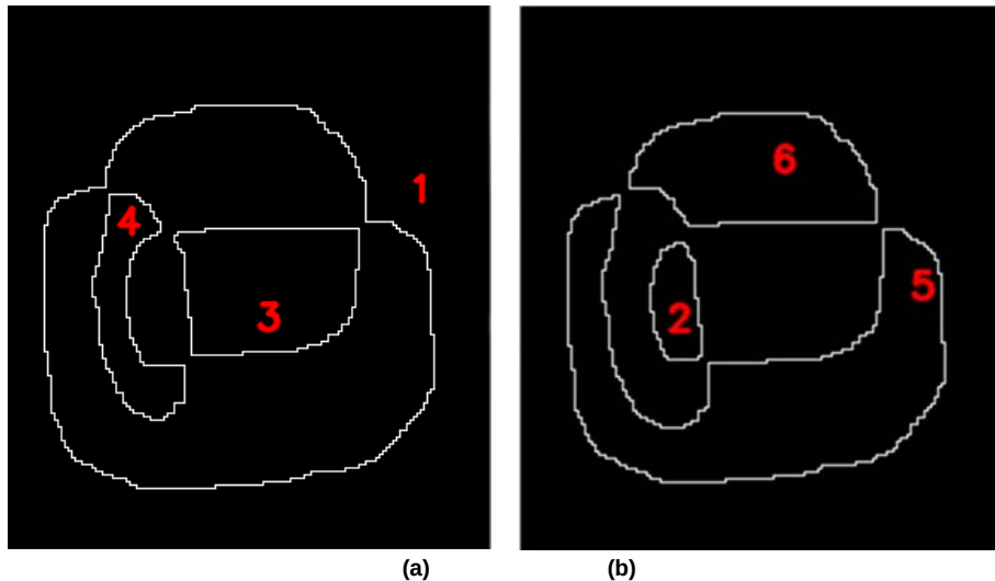
Fig. 6 Contour cycles constructed with region (cycle) numbers.
