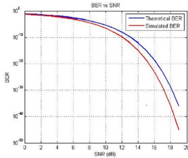
Figure3. BER of QPSK-OFDM with AWGN
