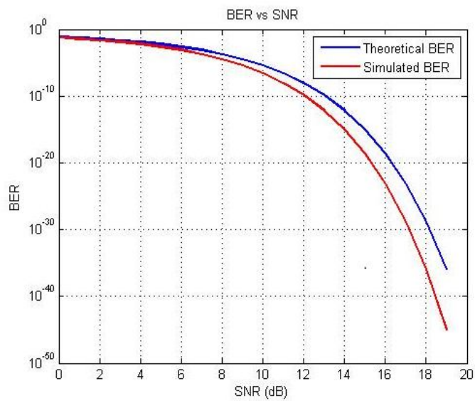
Figure4. BER of QPSK-OFDM with AWGN
