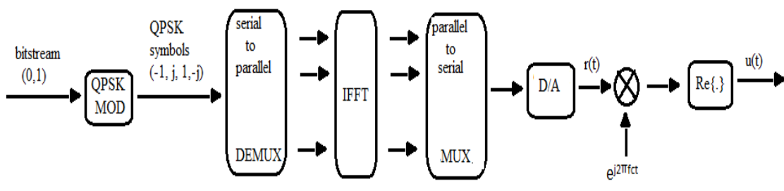
Fig. 3 OFDM Transmitter
