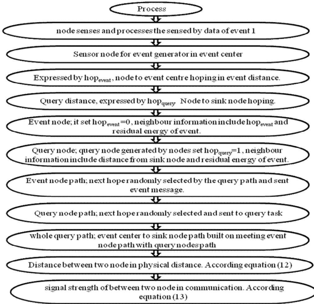
Flow sheet 1. Calculation of physical distance and signal strength between two nodes
