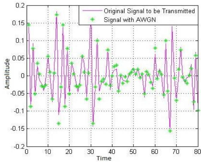
Figure 5. Generated OFDM Signal using MATLAB
