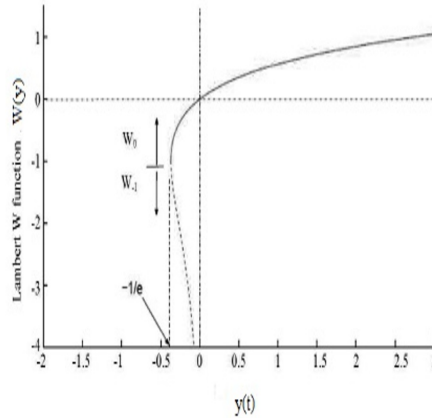
Fig. 1: Two real branches of the Lambert W function: the principal branch, k = 0 and k = -1 . Those two branches are used to identify the dominant characteristic roots of DDEs (Corless et al., (1996)).
