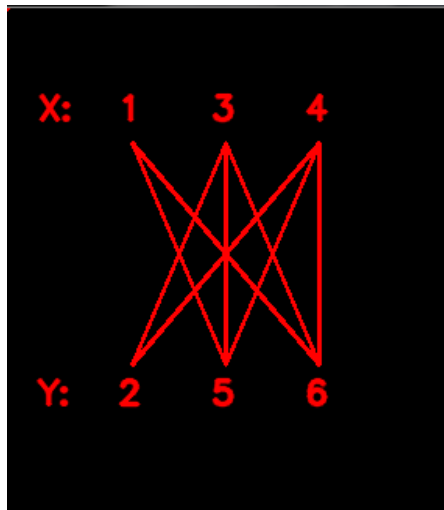
Fig. 9 Region graph bi-partitioned.
