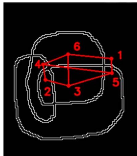
Fig. 10 Region (cycle) adjacency graph
