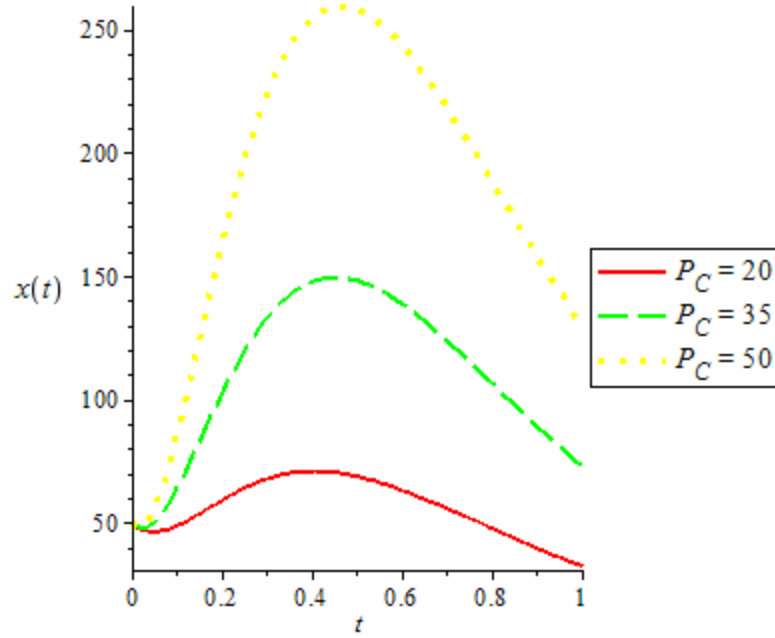
Figure 1: x(t) versus time t for various values of P_C at P_E = 10, K_1 = 0.02, K_2 = 0.33, \mu_C = 3, \mu_E = 2, \gamma = 2, \delta = 0.2, \omega = 0.04, v_0 = 0, x_0 = 50, y_0 = 300, z_0 = 10
