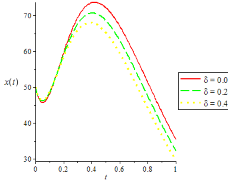
Figure 4: x(t) versus time t for various values of \delta at P_C = 20, P_E = 10, K_1 = 0.02, K_2 = 0.33, \mu_C = 3, \mu_E = 2, \gamma = 2, \omega = 0.04, v_0 = 0, x_0 = 50, y_0 = 300, z_0 = 10
