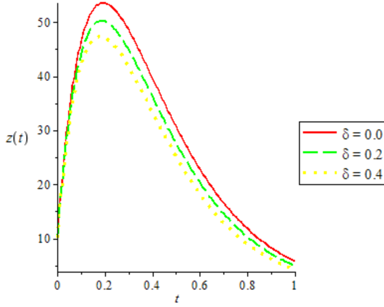
Figure 6: z(t) versus time t for various values of \delta at P_C = 20, P_E = 10, K_1 = 0.02, K_2 = 0.33, \mu_C = 3, \mu_E = 2, \gamma = 2, \omega = 0.04, v_0 = 0, x_0 = 50, y_0 = 300, z_0 = 10
