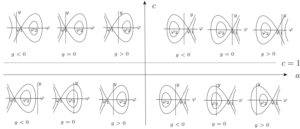
Figure 1: The phase portraits of system (9) under conditon (b + c)k < 0
