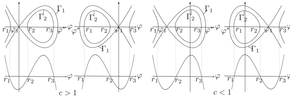
Figure 3: The phase portraits of homoclinic and periodic orbits under conditon g = 0
