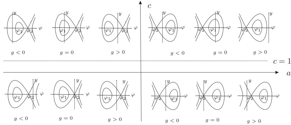
Figure 2: The phase portraits of system (9) under conditon (b + c)k > 0
