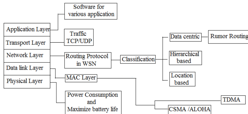
Figure1. OSI layers with corresponding protocols in WSN
