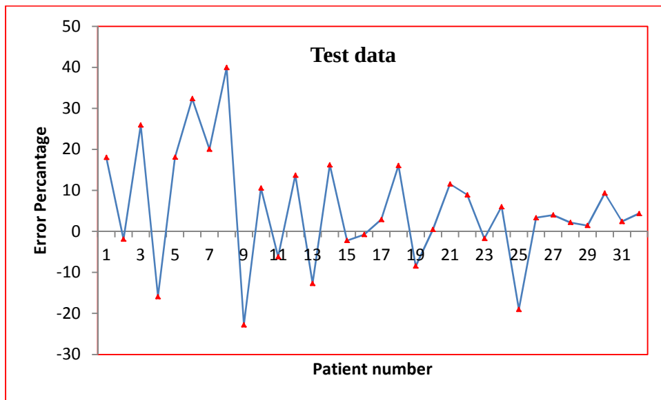
Figure 7: Error percentage \{(\text{error}/\text{measured}) \cdot 100\} of TAS values at 32 test data.
