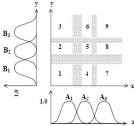
Figure 3: Corresponding fuzzy subspaces for a two-input Type-3 ANFIS with 9 rules
