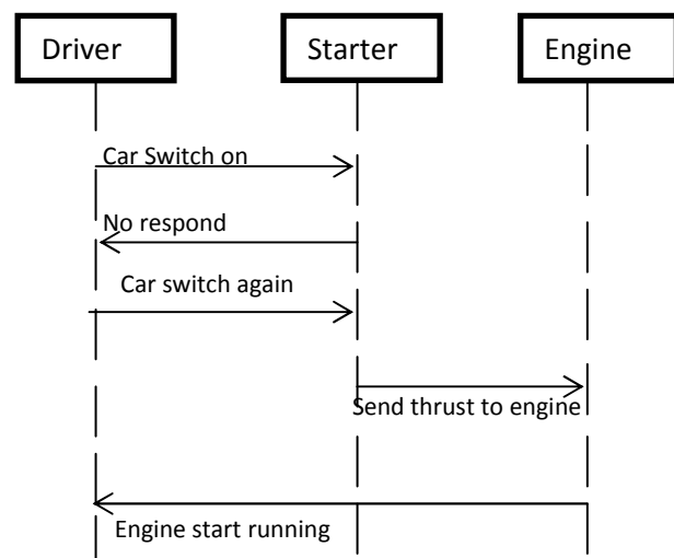
Figure 3 sequence diagram of a use case 'starting a Car'.
