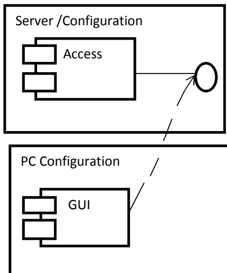
Figure 8: Deployment diagram of the of the component diagram in figure.
