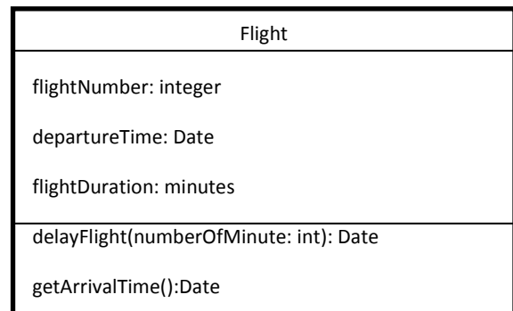
Figure 2: Class diagram for a class name Flight.
