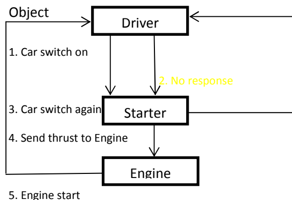
Figure 4: A Collaboration diagram for starting a car.
